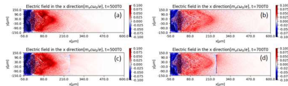
Figure 7. Two-dimensional spatial distribution of electric field intensity for ps laser-driven single and double-film targets. (a, b) Single target, (c, d) double-film target, (a, c) at 500T0, and (b, d) at 700T0.
