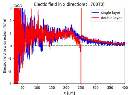
Figure 10. Electric field intensity distribution versus position for ps laser-driven single target and double-film target conditions. The data are from Figures 7(b) and 7(d). The blue line is for a single target and the red line is for a double-film target.
