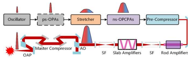
Figure 1. Schematic of the optical path of the SG-II peta-watt (SG-II PW) laser facility.
