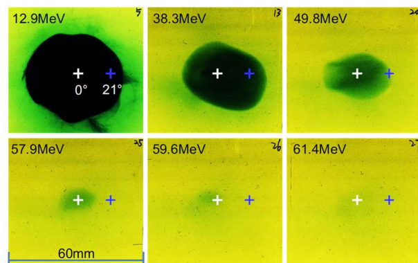
Figure 5. Several images of different layers of radiochromic film (RCF) sheets showing the proton signals with different proton energies.
