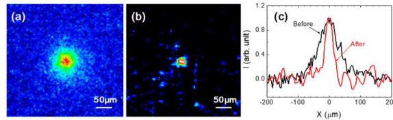
Figure 3. X-ray images and scanned intensity curve of laser irradiating metal planar target. (a) image before optimization; (b) image after optimization; (c) scanned intensity curve along the x-direction.
