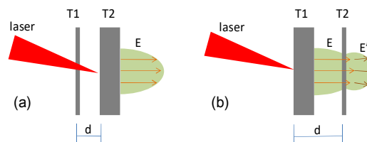
Figure 6. Two different double target structures. (a) Double-layer target for plasma mirror. (b) Double-film target for modulating sheath field modulation.
