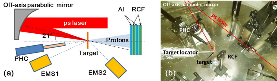
Figure 4. Light path and diagnostic arrangement of laser-driven proton acceleration (LDPA) experiment based on the target normal sheath acceleration (TNSA) mechanism. (a) Schematic of arrangement. (b) Photograph of the target chamber.
