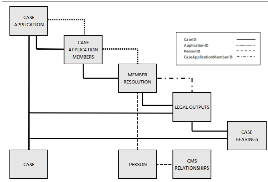
Figure 1: Structure of the CMS, including linkages between tables
