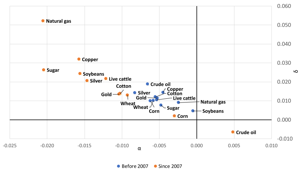
Fig. 9. Alpha-Delta-before/since.
