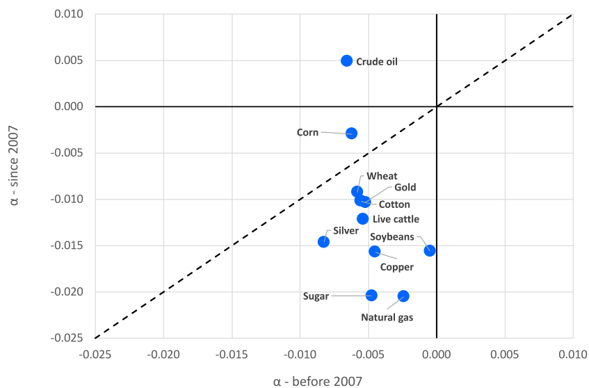
Fig. 7. Alpha-Alpha relationship.
