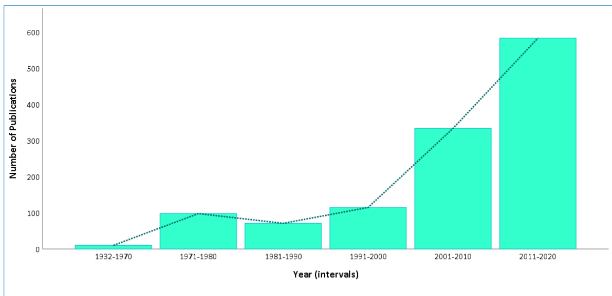
Figure 15. Bar chart of number of shark publications by decade.
