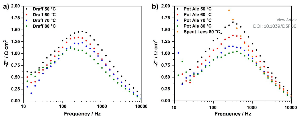
Figure 9. Temperature-sweep Bode format EIS for PEMECs operating with (a) a digested draff (D4)-PMA anolyte solution and (b) digested pot ale (PA2)-PMA and spent lees (SL2)-PMA anolyte solutions, collected at 850 mV using H 2 SO 4 as a catholyte.
