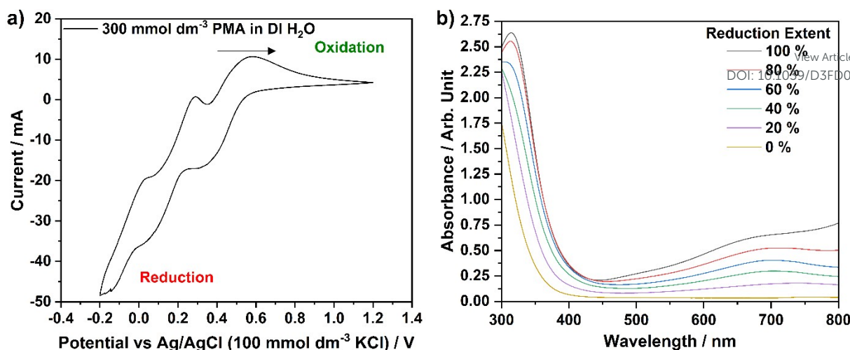
Figure 5. (a) CV plot of a 300 mmol dm -3 solution of H 3 [PMo 12 O 40 ]·25.1H 2 O (in DI H 2 O), collected between -200 mV and 1200 mV vs a Ag/AgCl reference electrode and (b) UV-visible spectra of PMA solution reduced by 0, 20, 40, 60, 80 and 100 %, with respect to the first two-electron process, through chronoamperometric experiments.
