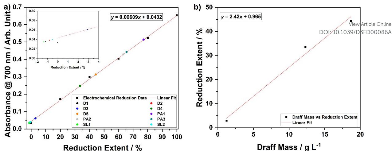
Figure 6. (a) A calibration curve (absorbance at 700 nm vs percentage reduction of PMA) with overlain data points for thermally digested whisky co-products, Inset: magnified region showing the negligible extent of reduction of digested draff and pot ale samples, and (b) a plot of percentage reduction of PMA versus draff concentration (dry basis), used to determine that 40.9 g L -1 of 'dried' draff should be required to reduce PMA by two electrons.
