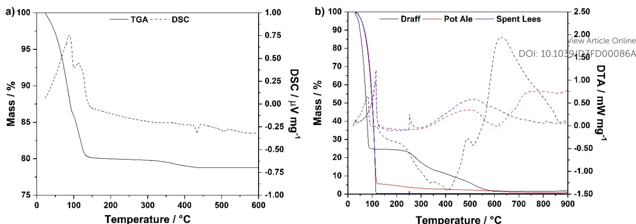
Figure 3. (a) Simultaneous thermal analysis plots (STA) for H_3[PMo_{12}O_{40}] \cdot xH_2O , indicating that the material contains 25.1 moles of water of crystallisation, and (b) STA plots for draff, pot ale and spent lees whisky co-products from the Isle of Raasay Distillery.
