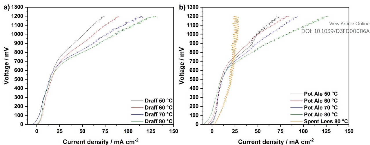
Figure 7. Temperature-sweep VI curves for PEMECs operating with (a) a digested draff-PMA anolyte solution and (b) digested pot ale-PMA and spent lees-PMA anolyte solutions, collected at 850 mV using \text{H}_2\text{SO}_4 as a catholyte.
