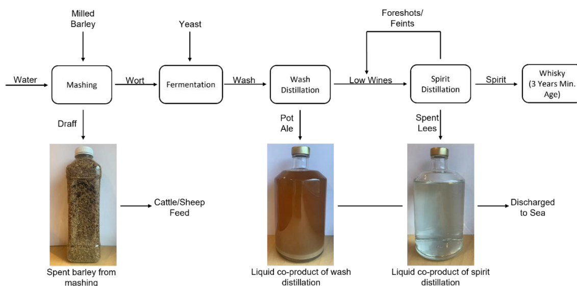
Figure 1. A basic flow-diagram of the whisky production process and the co-products generated as a result.
