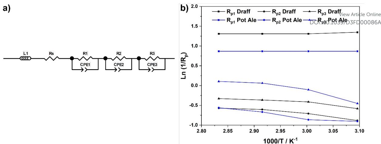
Figure 10. (a) Equivalent circuit model employed to determine fitting parameters for the EIS presented in figure 8 and (b) Arrhenius-style plots of \ln(1/R_p) versus 1000/T for resistance data obtained from ECF of EIS.
