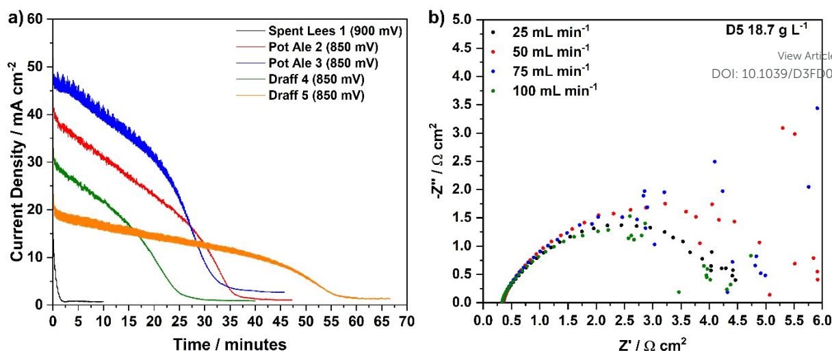
Figure 11. (a) Chronoamperometric data for the PEMECs operating on digested draff-PMA, pot ale-PMA (850 mV) and spent lees-PMA (900 mV) anolyte solutions during gas evolution experiments and (b) EIS collected for PEMEC3, operating on a draff (D5)-PMA anolyte, illustrating the effect of peristaltic pump flow rate on the spectrum quality.
