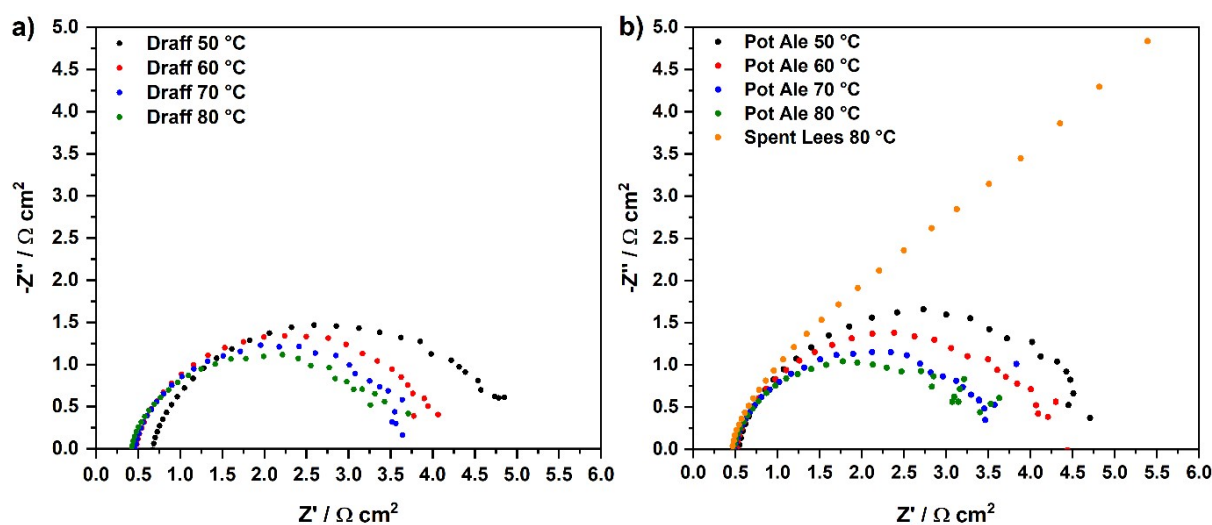
Figure 8. Temperature-sweep complex plane EIS for PEMECs operating with (a) a digested draff (D4)-PMA anolyte solution and (b) digested pot ale (PA2)-PMA and spent lees (SL2)-PMA anolyte solutions, collected at 850 mV using \text{H}_2\text{SO}_4 as a catholyte.
