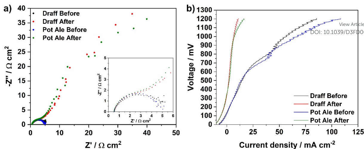
Figure 12. Complex plane EIS for PEMEC2 operating with digested draff (D4)-PMA and pot ale (PA2)-PMA anolyte solutions, collected at 850 mV before and after chronoamperometry experiments, and (b) VI curves for PEMEC2 operating with the same anolyte solutions, before and after chronoamperometry experiments at 80 °C using H 2 SO 4 as a catholyte.
