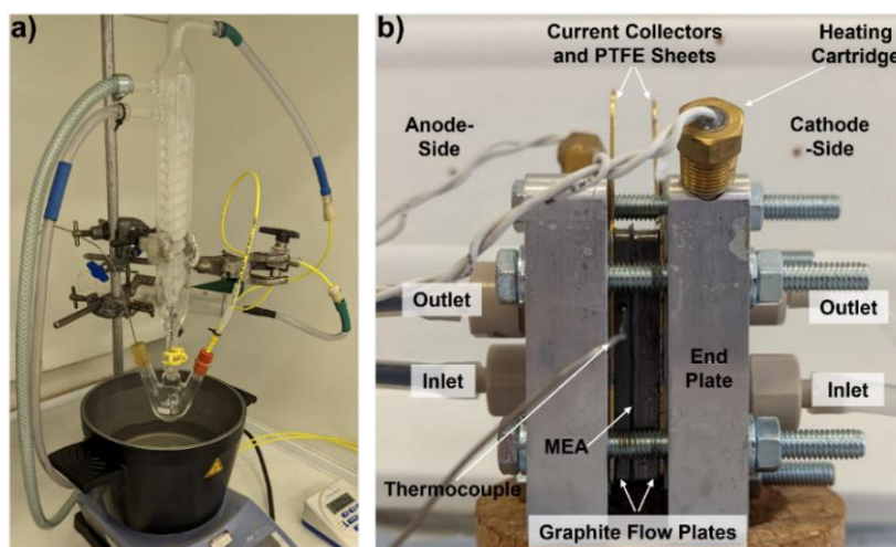
Figure 2. (a) Image of the setup employed to thermally digest biomass using the PMA catalyst and (b) a labelled image of the PEM flow cell used for electrolysis experiments.
