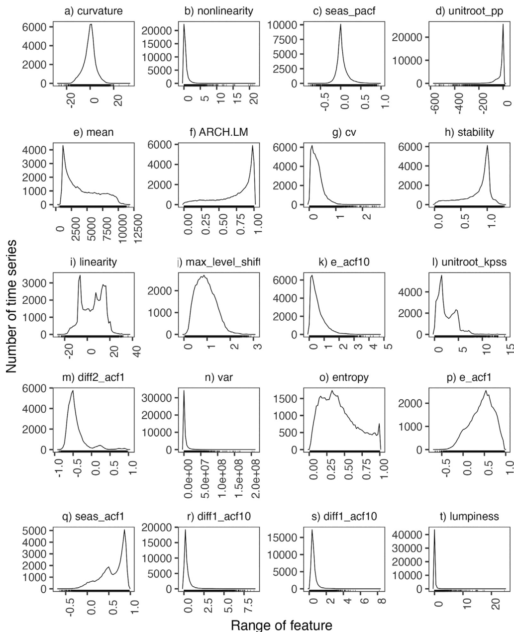
Fig. 3. Features of monthly time series from M4 competition dataset.
