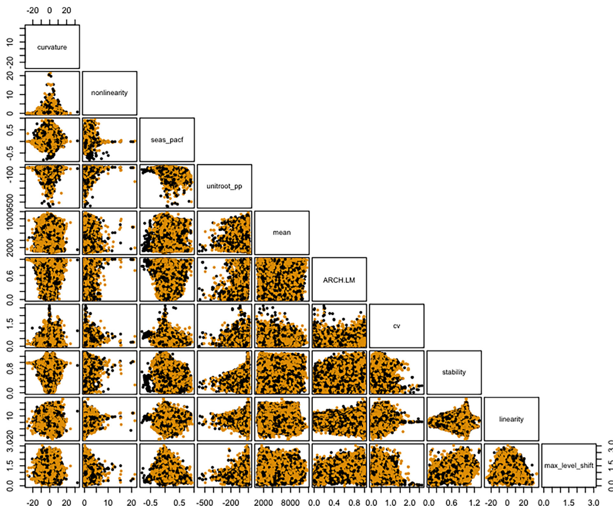
Fig. 9. Time series features matrix. Each point indicates one single time series with a feature in x-axis and another at y-axis. The black and yellow colors show the outperformance of AD and AF, respectively.
