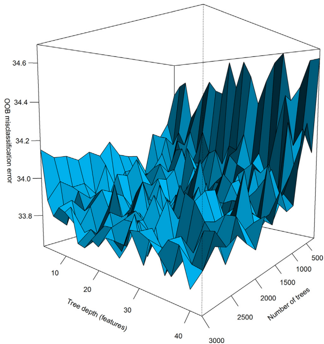
Fig. 12. Surface plot of the number of features (depth), number of trees and misclassification error of random forest model.
