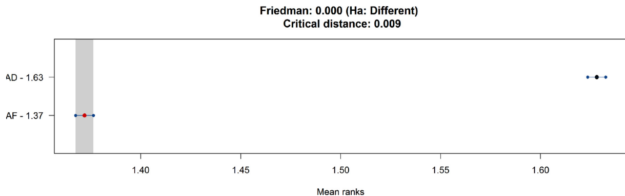
Fig. 8. Performance of AF and AD models evaluated using MCB test. RMSSE values are used for computing the ranks and a 95 percentile confidence level.
