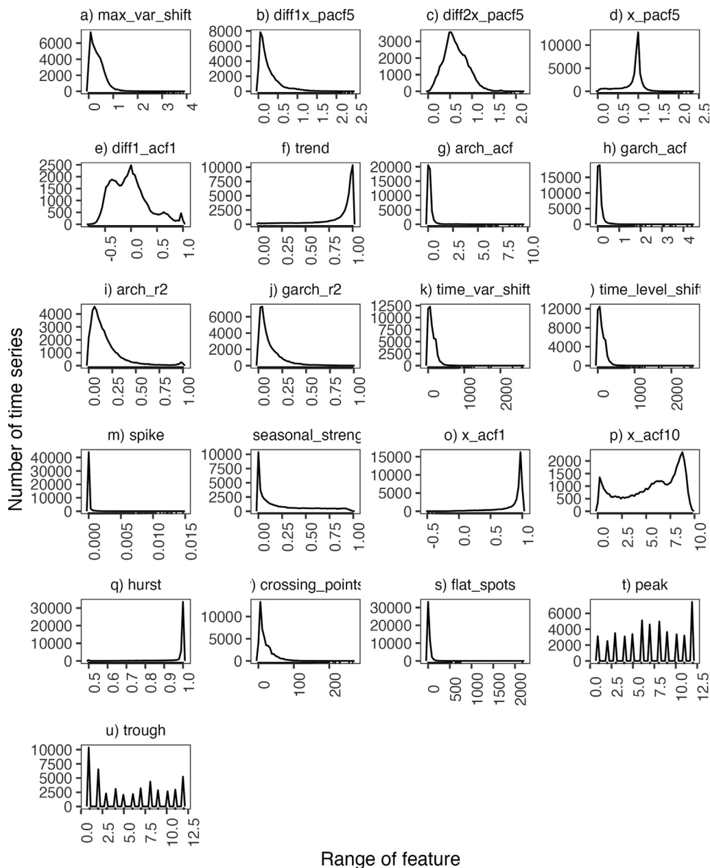
Fig. 4. Features of monthly time series from M4 competition dataset (continue).
