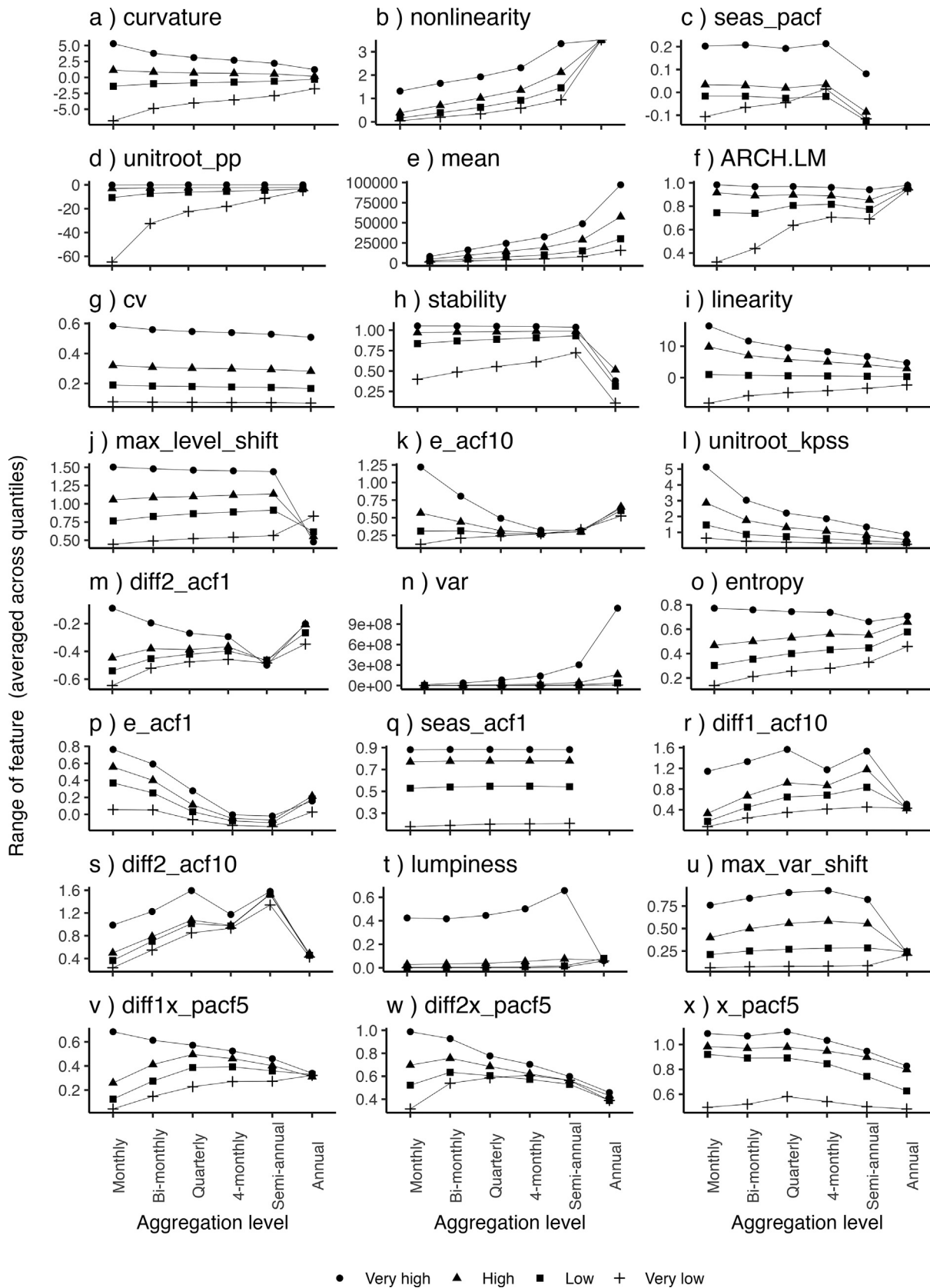
Fig. 5. The effect of non-overlapping temporal aggregation on monthly time series features of M4 competition dataset.
