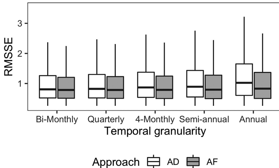
Fig. 7. RMSSE errors through aggregation levels.
