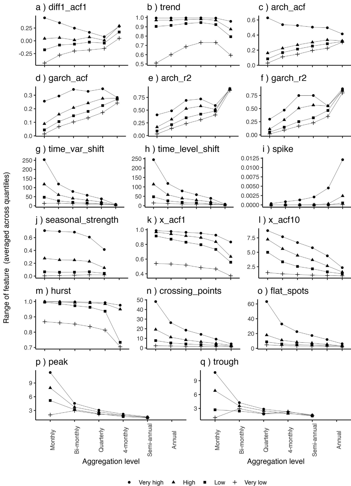
Fig. 6. The effect of non-overlapping temporal aggregation on monthly time series features of M4 competition dataset (continue).
