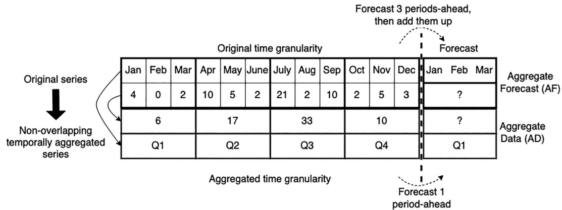
Fig. 1. Aggregate forecast vs. aggregate data approaches. Assuming a monthly time series is available and a forecast over one quarter (aggregation level = 3 months) is required. We first generate forecast for 3 periods ahead and then sum them up to create forecast over the quarter (Forecast by AF approach). Then, we create the temporally aggregated series by dividing the original series into the block of 3 periods. Next, we forecast for 1 period ahead (Forecast by AD approach).
