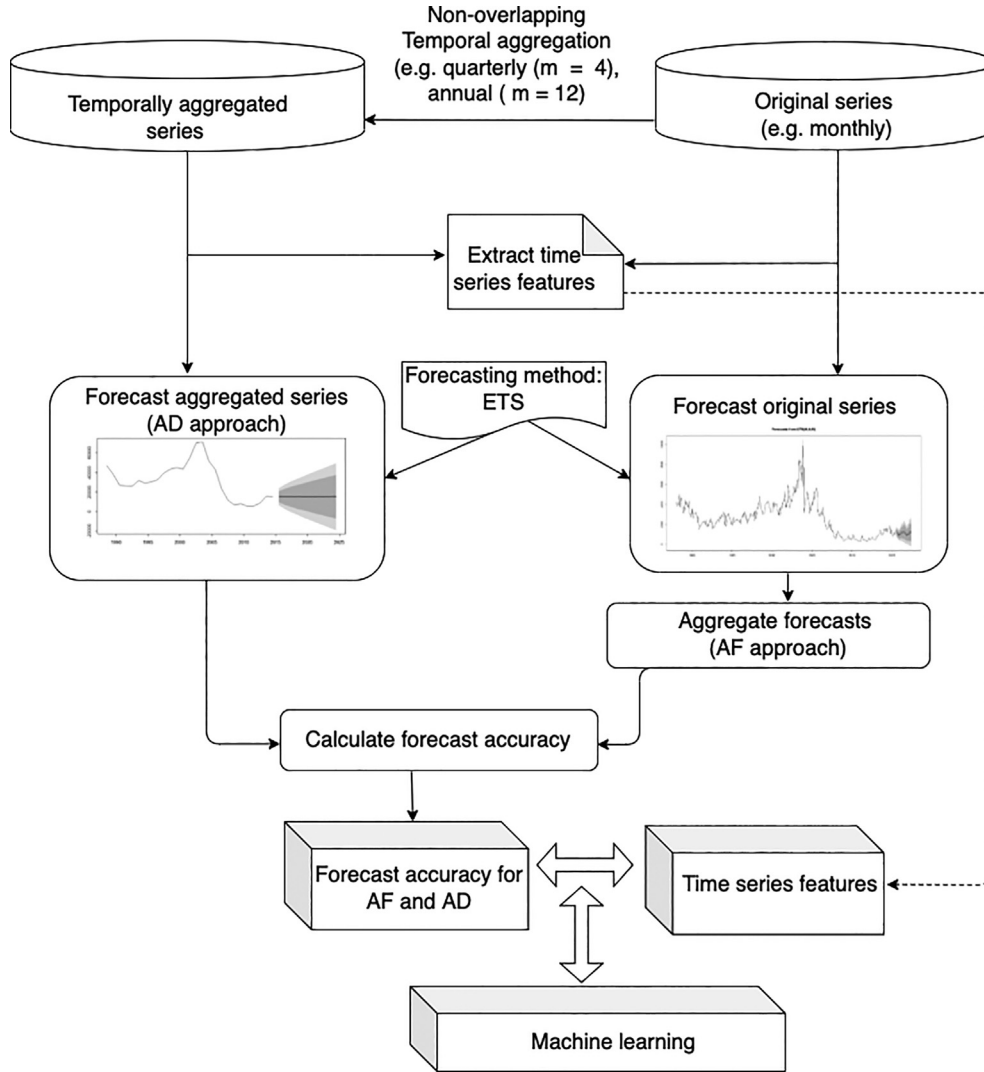
Fig. 2. Design of the experiment framework.
