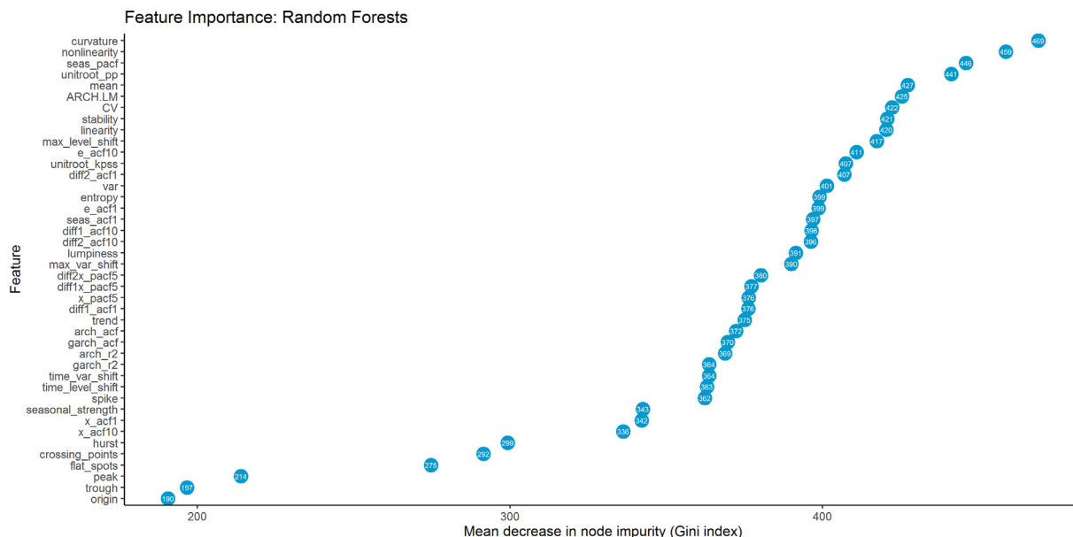
Fig. 14. Predictor features importance spectrum for the M4 data. A feature importance is computed using the mean decrease in Gini index.
