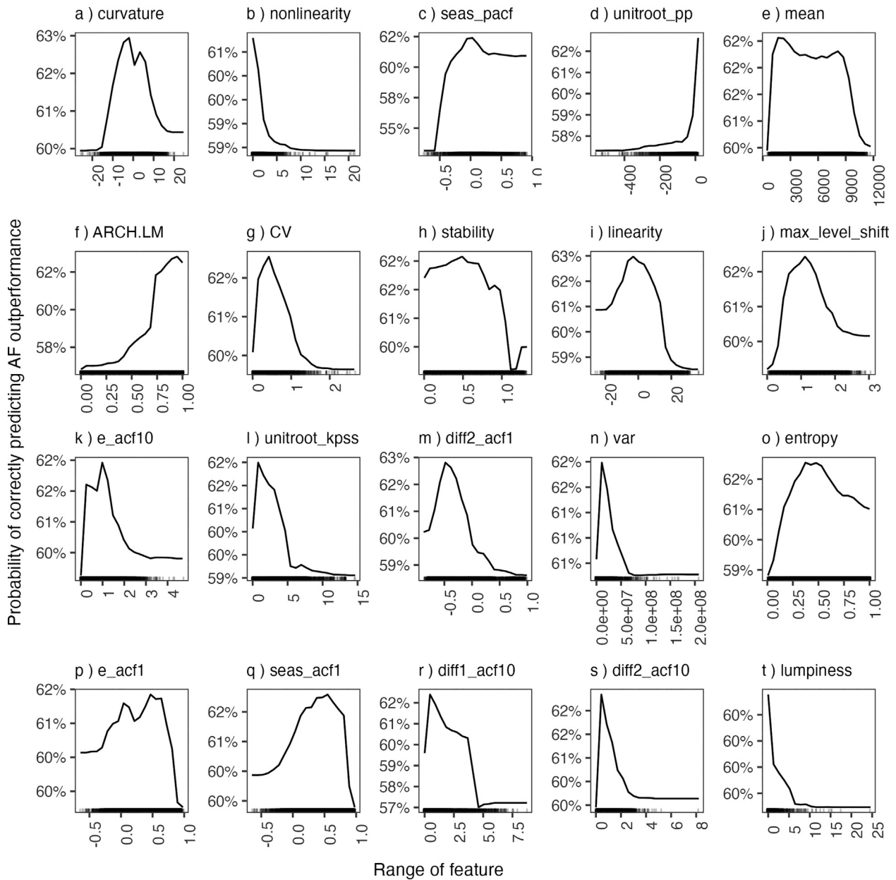
Fig. 15. Partial dependence plot - the range of features vs. the probability of classifying AF versus AD.
