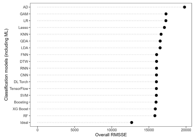
Fig. 11. Utility accuracy comparison.
