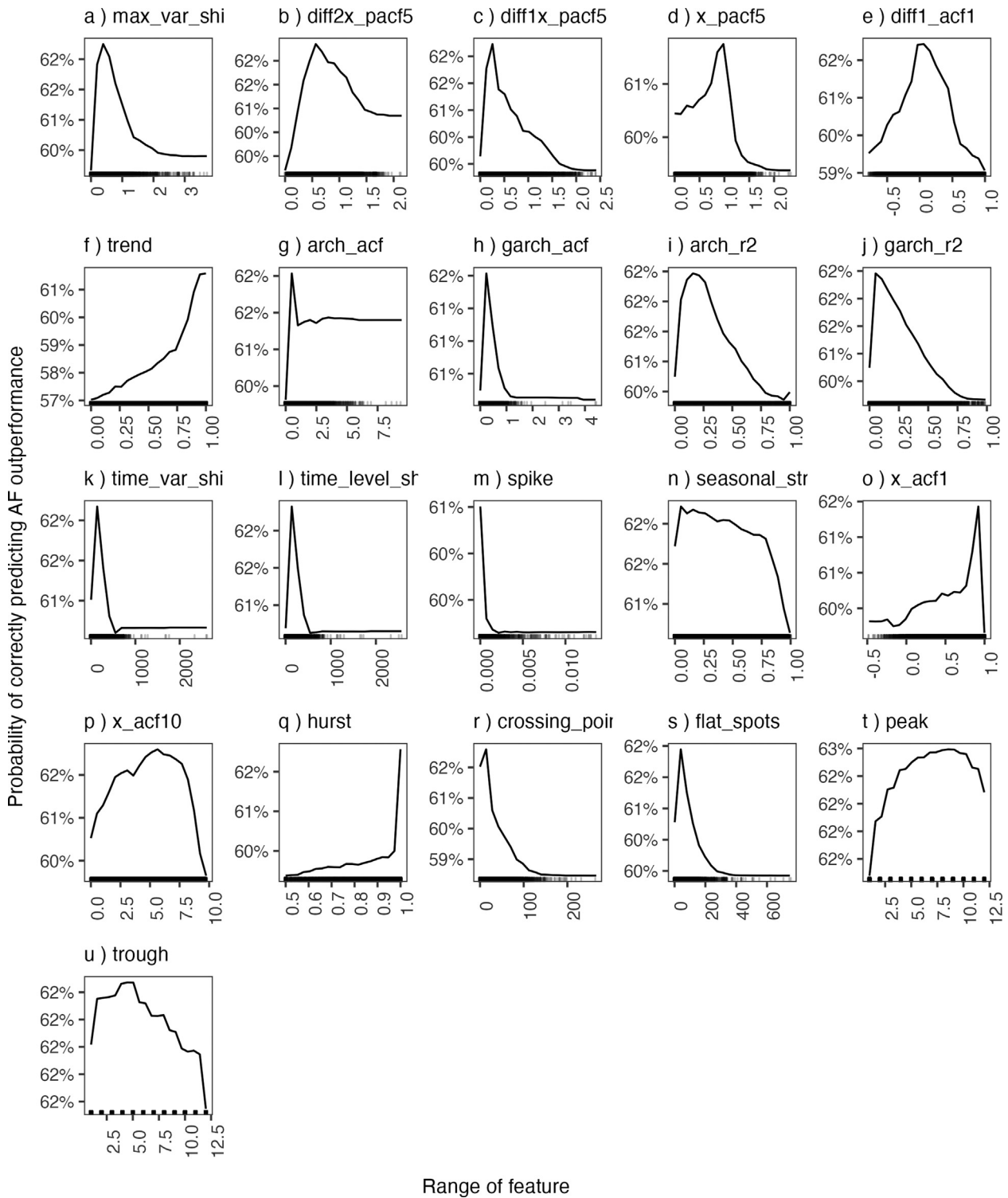
Fig. 16. Partial dependence plot - the range of features vs. the probability of classifying AF versus AD (continue).
