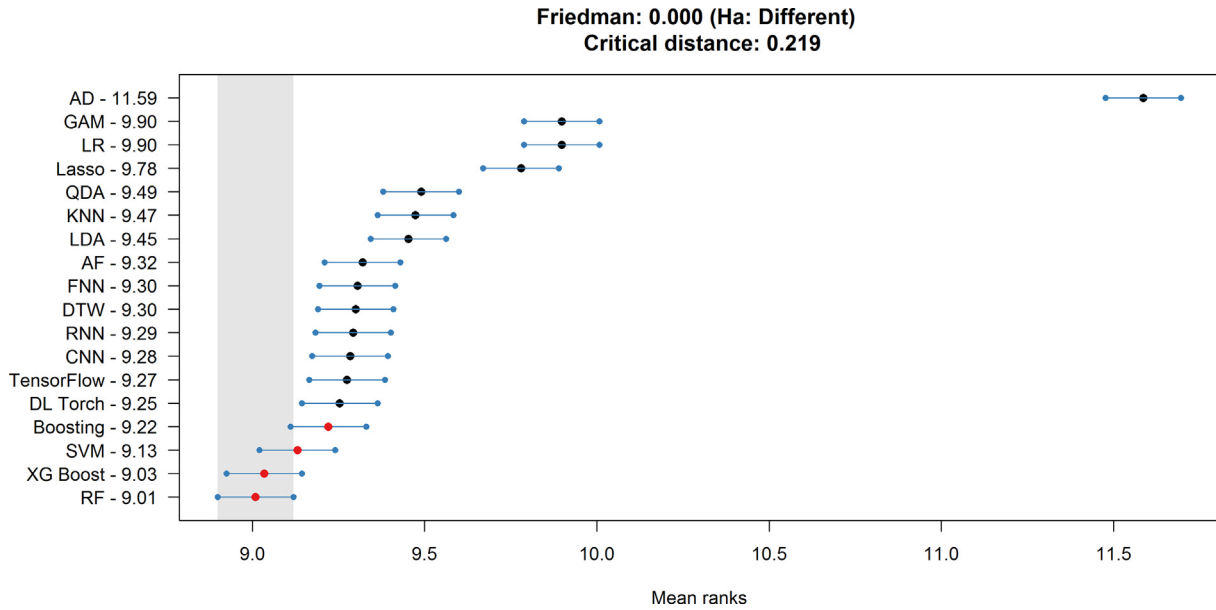
Fig. 10. Performance of different models evaluated through MCB test. RMSSE errors are used for computing the ranks and a 95 percentile confidence level.
