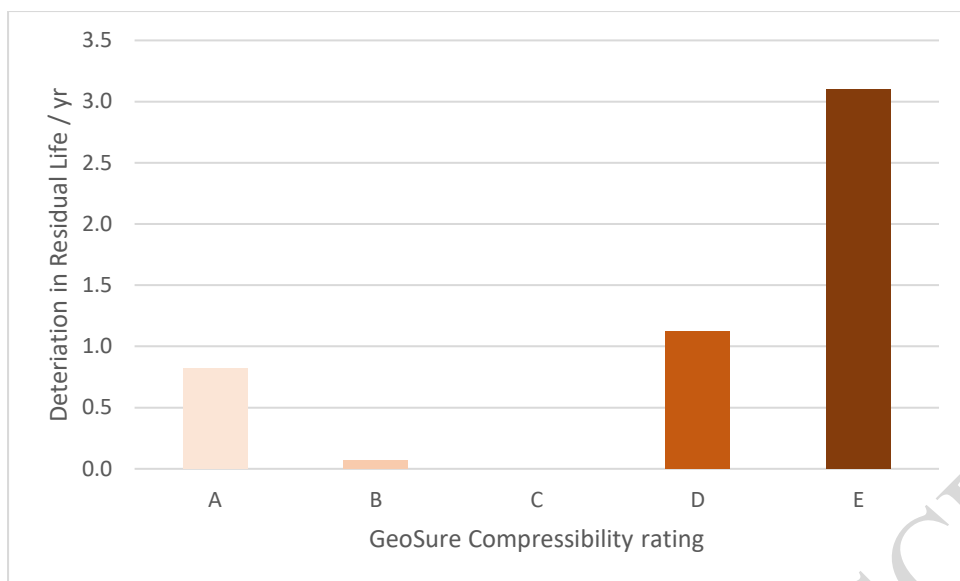
Figure 16 GeoSure Compression values against the Residual Life deterioration rates (all roads)
