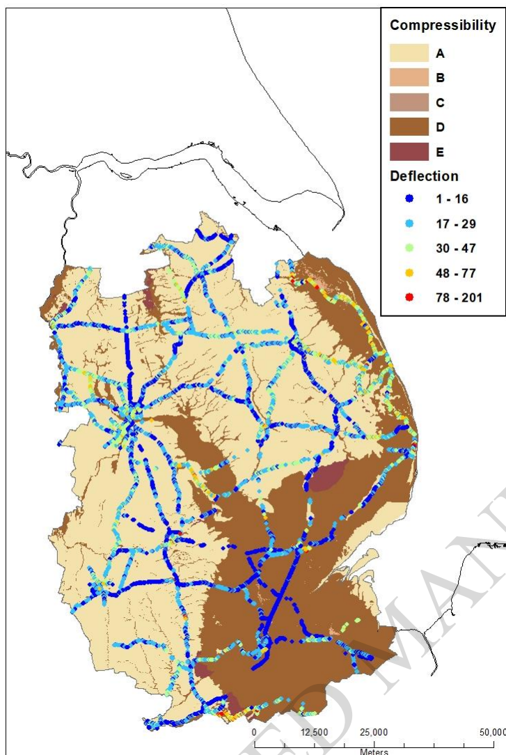
Figure 15 Lincolnshire County Council deflectogram survey residual life data for 2010 to 2013 and the BGS GeoSure compressibility susceptibility map. © Lincolnshire County Council. Contains Ordnance Survey data © Crown copyright and database right [2022]
