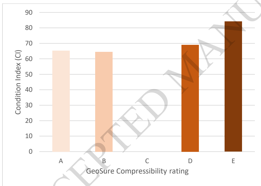
Figure 17 Average Condition Index (CI) between 2010 and 2013 of all surveyed Lincolnshire roads in areas with GeoSure compressibility rating of A to E.
