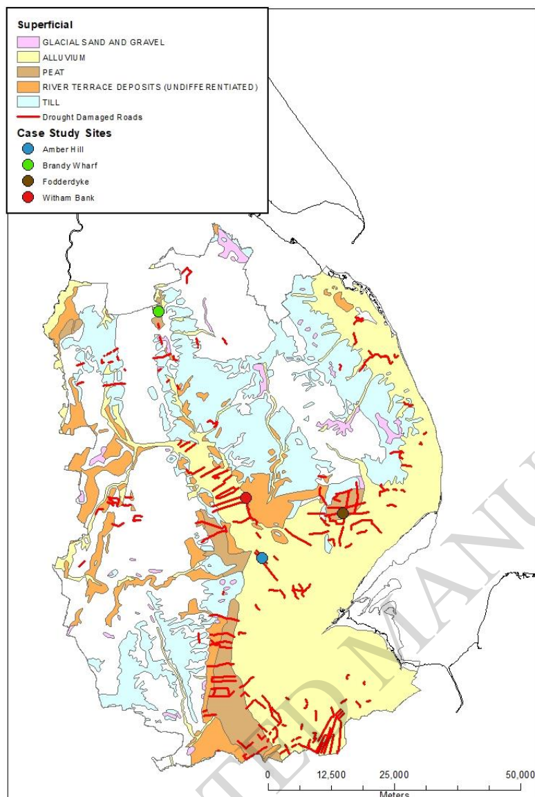
Figure 18 Drought related subsidence claims in Lincolnshire 2011 and the BGS 625k superficial geology map. © Lincolnshire County Council. The four case study sites are highlighted by the coloured dots. N.B. The 625k scale generalised superficial geological map compiles alluvium and tidal flat deposits as Alluvium. Contains Ordnance Survey data © Crown copyright and database right [2022]
