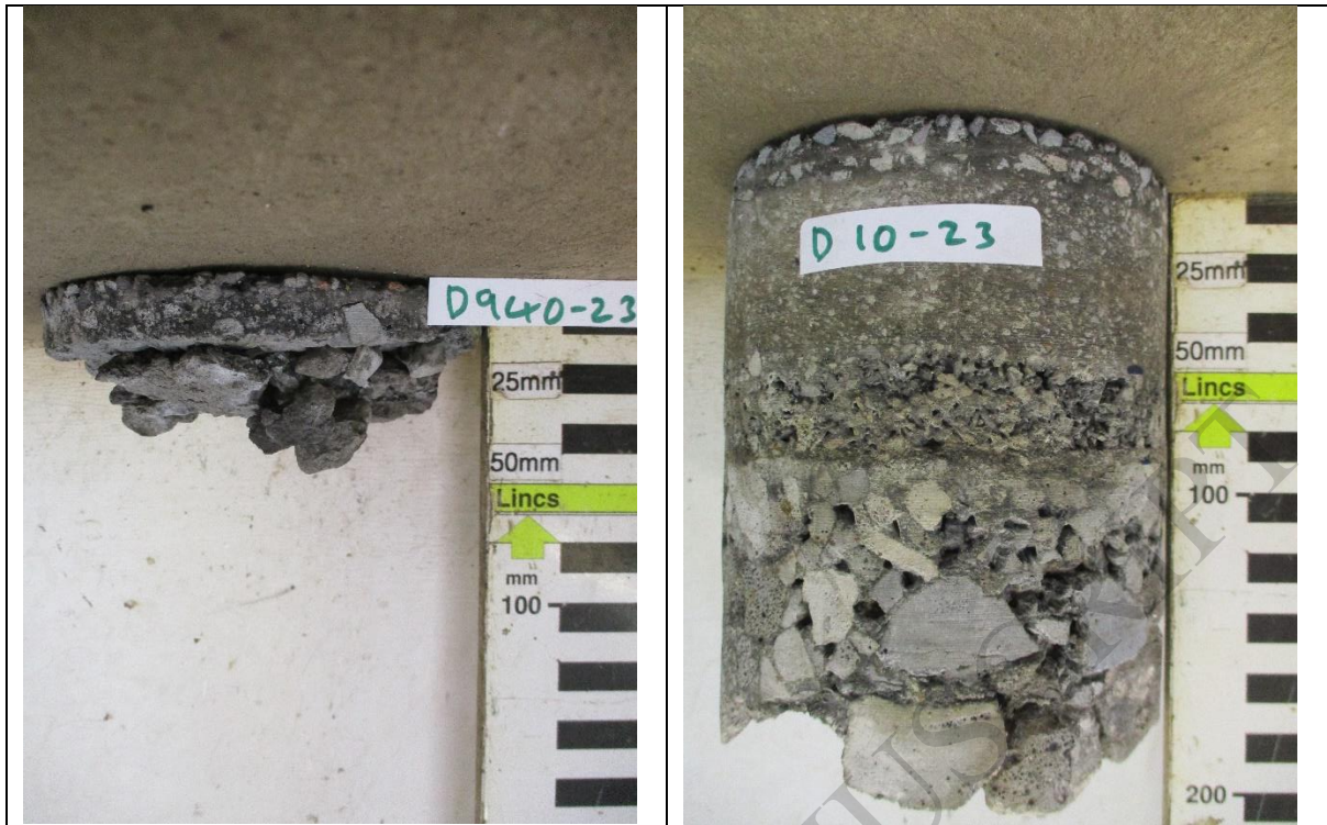
Figure 4: Typical depths of 'evolved' road foundations in the county. Left: Chalk Lane, Withern has a depth of 2.5 to 5 cm, and Church Lane in Friskney has a depth of 20 cm. At least 4 surface courses can be seen to have been added at Friskney.
