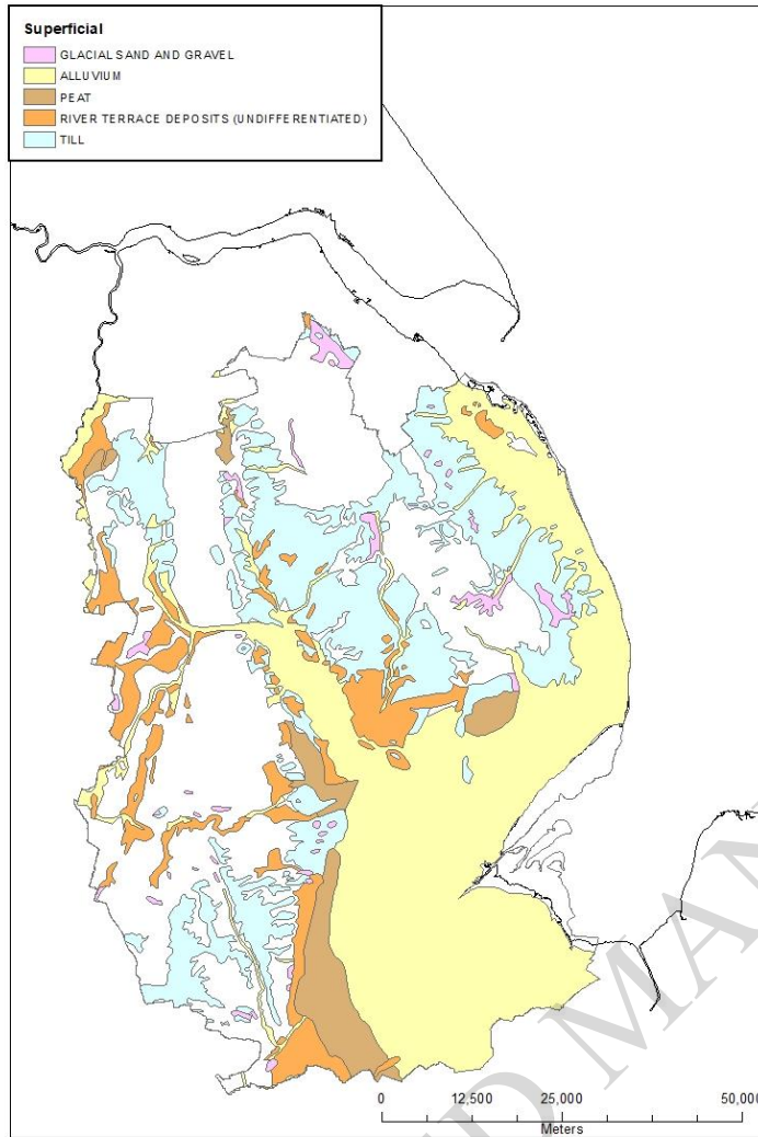
Figure 2 Superficial geology of Lincolnshire (BGS Geology 625K). Contains Ordnance Survey data © Crown copyright and database right [2022]
