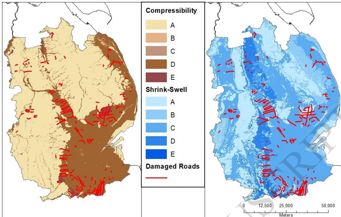
Figure 19 GeoSure Compressibility and clay shrink-swell with sites recorded (red lines) by LCC as requiring remedial work due to drought damage during 2011-2012. © Lincolnshire County Council. Contains Ordnance Survey data © Crown copyright and database right [2022]
