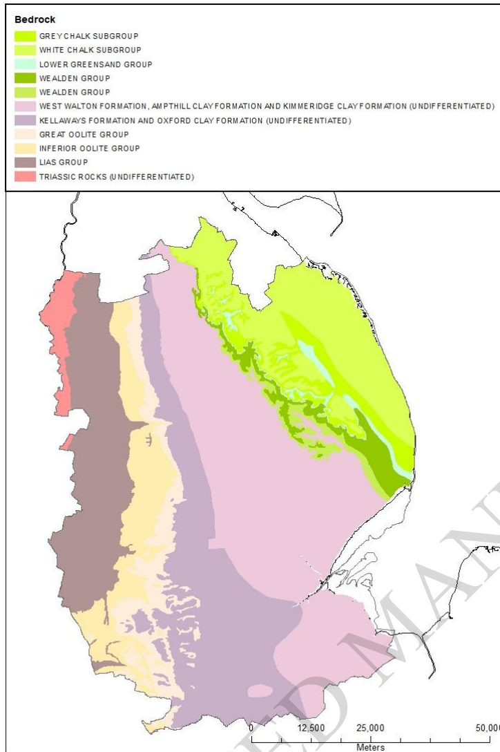
Figure 3 Bedrock geology of Lincolnshire County Council county (BGS Geology 625K). Contains Ordnance Survey data © Crown copyright and database right [2022]
