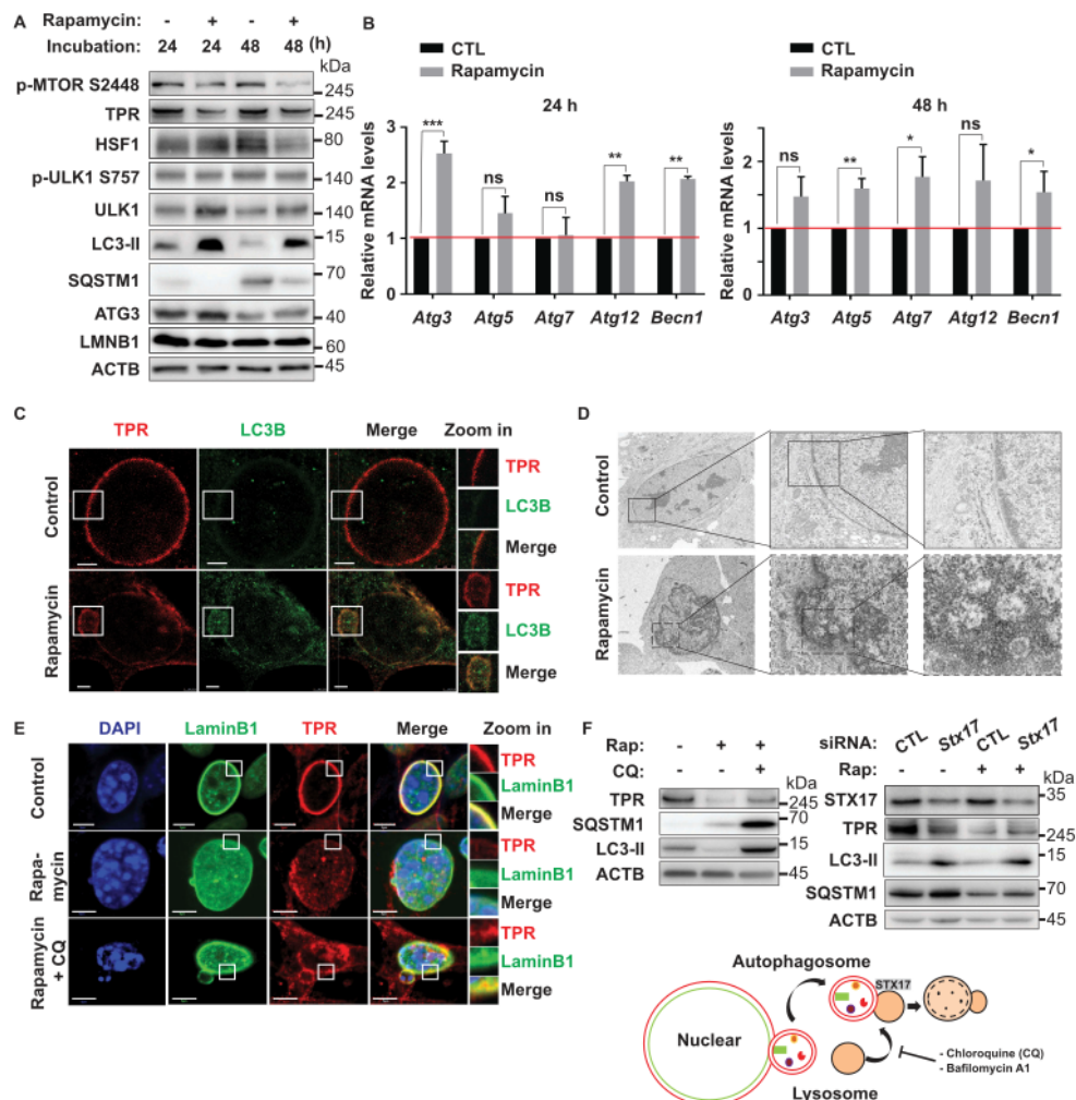
Figure 4. MTOR inhibition depleted TPR expression in vitro and induced nucleophagy. (A) Western blotting analysis of Vn19 cells treated with DMSO or rapamycin for 24 or 48 h. (B) Q-RT PCR analysis of autophagy related genes in Vn19 cells treated with DMSO or 10 nM rapamycin. Data show mean \pm SD from three independent experiments ( n = 3 ). P values are based on Student's t -test with (***) indicating P < 0.001 . (C) STED – immunostaining analysis of LC3B and TPR in Vn19 cells treated with DMSO or 10 nM rapamycin. Cell membrane blebbing were highlighted in the square (scale bar: 2.5 \mu m). (D) TEM analysis of Vn19 cells treated with either DMSO or 10 nM rapamycin. Autophagic vacuoles are indicated by arrows and highlighted on the right. (E) Vn19 cells treated with rapamycin or rapamycin + chloroquine (CQ) and stained with nuclear envelope protein LMNB1 and TPR. Treatment with CQ could recover TPR expression (scale bar: 5 \mu m). (F) Western blotting analysis of TPR, SQSTM1, and LC3B protein expression in Vn19 cells treated with CQ or siStx17 in the absence and presence of rapamycin treatment.
