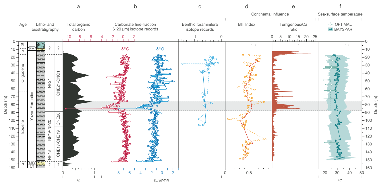
Fig. 3 | Inorganic and organic geochemical records from the Mossy Grove Core (MGC) in the depth domain. a Total organic carbon 87 . b Carbonate fine-fraction (<20 μm) δ 13 C and δ 18 O and (c) benthic foraminifera δ 18 O records. Indicators of continental influence. d Branched and Isoprenoid Tetraether (BIT) index. e Terrigenous/Ca ratio. Sea-surface temperature. f TEX 86 (filled markers represent
