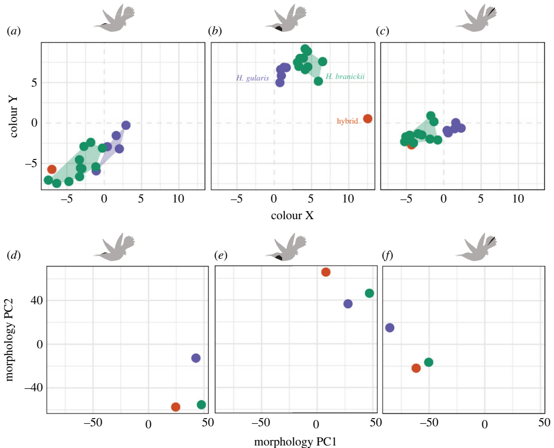
Figure 3. Colour and morphological divergence in Heliodoxa hummingbirds. Plots show perceptually uniform [82] avian tetrahedral colour space coordinates (a–c) and principal components (PC) axes 1 and 2 for feather morphological data (d–f) in crown (a,d), gorget (b,e) and tail feathers (c,f). Point colours correspond to Heliodoxa branickii (green), Heliodoxa gularis (purple) and the Heliodoxa backcross hybrid (orange).
