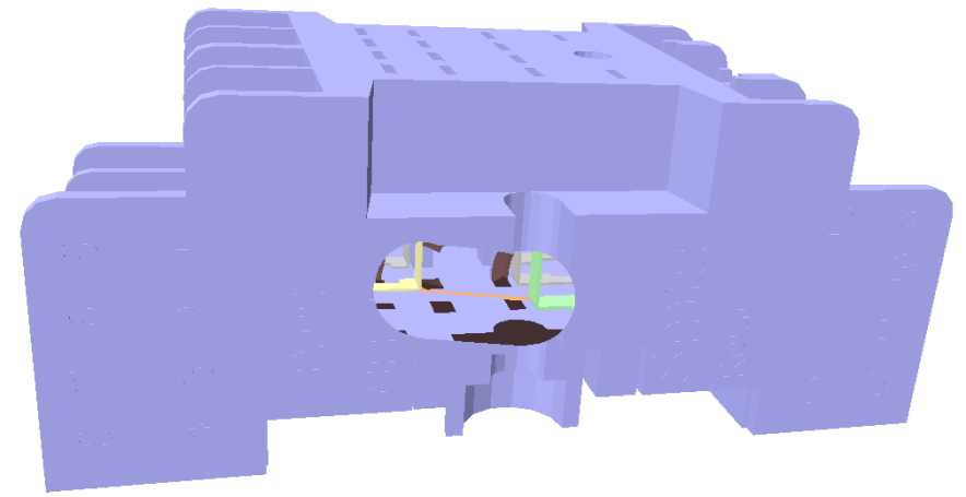
Example of a Path Window. A certain section around the displayed path is automatically cut out of the assembly to see through occluding components
