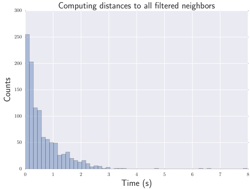
FIGURE 7.7: Time for computing distances from all filtered segments.
