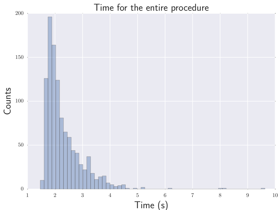
FIGURE 7.1: Global times for selecting next segment.
