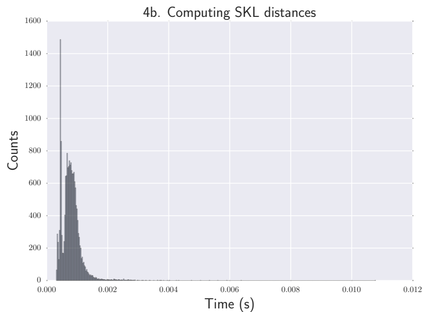
FIGURE 7.6: Time for computing symmetric Kullback-Leibler divergence between the single Gaussian distributions of the MFCCs values of two excerpts.
