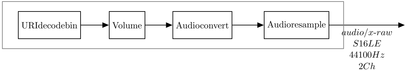
FIGURE 6.1: Custom audio bin, that corresponds to an audio player only responsible for the playback of a single excerpt.
