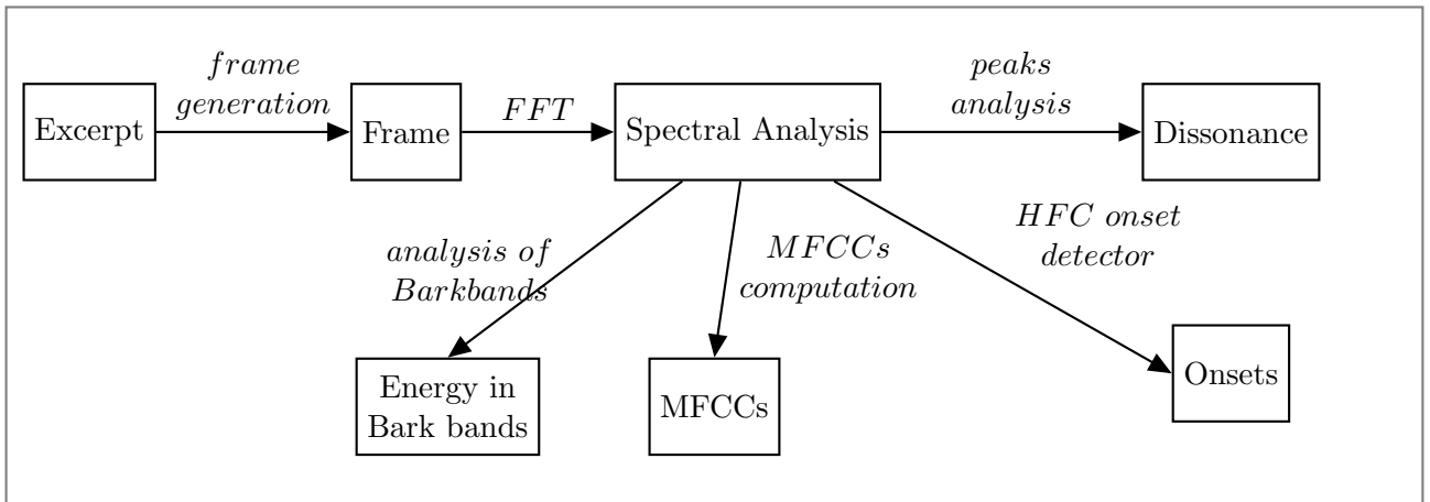
FIGURE 5.2: Schema for the extraction of low level audio features from excerpts.
