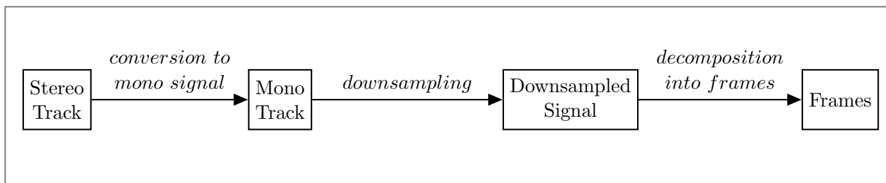
FIGURE 2.2: Standard procedure preliminary to the extraction of audio features.
