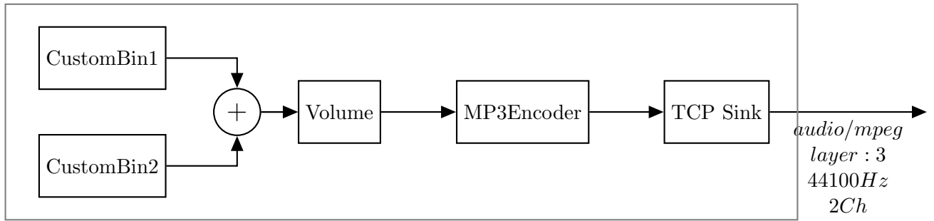
FIGURE 6.2: Schema for the audio player implemented.
