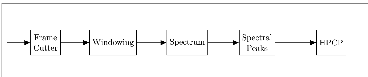
FIGURE 2.5: Computation of HPCP with Essentia. Each block corresponds to a different algorithm of Essentia.
