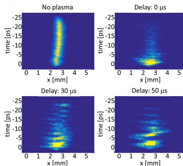
Figure 2. Streaked bunch measurement for varying delay of bunch arrival w.r.t. discharge pulse. The color scale is different for the measurement without plasma in comparison to the others to have good visibility for all cases.
