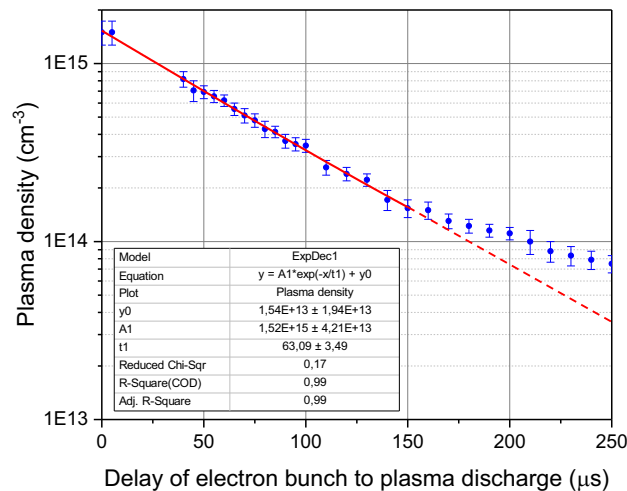
Figure 4. Plasma density vs. delay of the electron bunch with respect to the discharge pulse.
