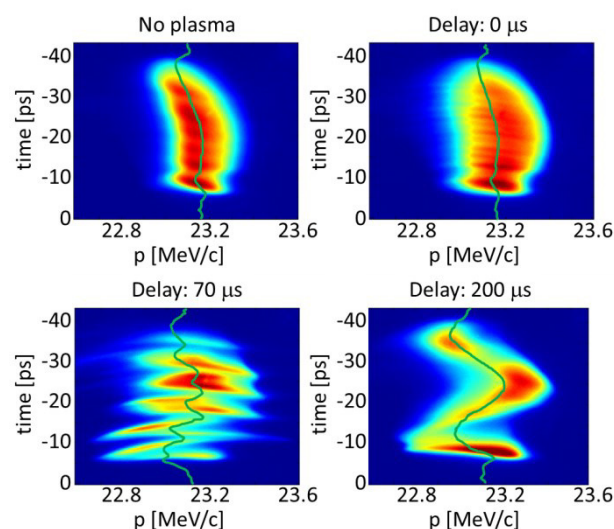
Figure 3. Longitudinal phase space for varying delay of bunch arrival w.r.t. discharge pulse.
