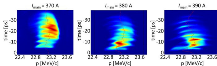
Figure 5. Longitudinal phase space for three different currents of the focusing solenoid.
