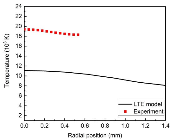
Figure 3. Radial plasma temperature obtained in the LTE model for an arc in \text{CO}_2 and the plasma temperature from OES for an arc current of 200 A at axial position 1 mm away from the cathode tip.
