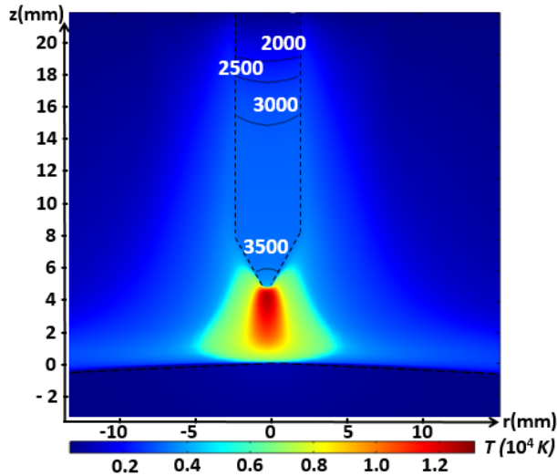
Figure 2. Two-dimensional distribution of the plasma temperature and the temperature in the electrodes obtained with the LTE model for an arc in \text{CO}_2 at current of 200 A.
