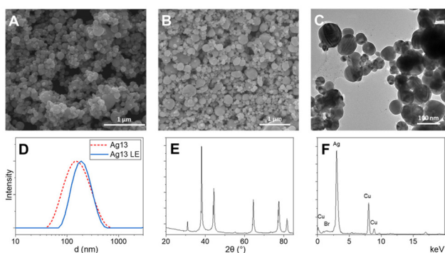
Fig. 3 (A) SEM micrograph of sample Ag13 ( \text{AgNP}@ \epsilon\text{-Ahx} ); (B and C) SEM and TEM images of sample Ag13LE ( \text{AgNP}@ \text{PEDOT:PSS} ); (D) DLS spectra of sample Ag13 ( \text{AgNP}@ \epsilon\text{-Ahx} , red dotted line) and Ag13LE ( \text{AgNP}@ \text{PEDOT:PSS} , blue line); (E) XRD spectra of sample Ag13LE ( \text{AgNP}@ \text{PEDOT:PSS} ); (F) EDX spectra of sample Ag13LE ( \text{AgNP}@ \text{PEDOT:PSS} ).
