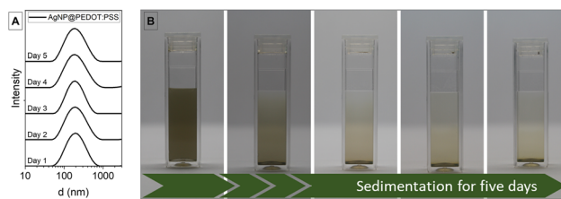
Fig. 4 (A) Hydrodynamic diameter of \text{AgNP}@ \text{PEDOT:PSS} determined by DLS, showing stability for 5 days; (B) visible sedimentation of redispersed diluted \text{AgNP}@ \text{PEDOT:PSS} dispersions.
