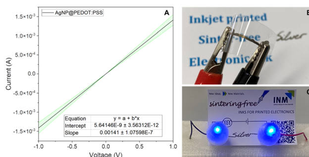
Fig. 5 (A) Voltage–current curve measured on deposited \text{AgNP}@ \text{PEDOT:PSS} ; (B) image of \text{AgNP}@ \text{PEDOT:PSS} deposited on bendable substrate (PET); (C) image of deposited \text{AgNP}@ \text{PEDOT:PSS} on paper and connected into a circuit with LEDs and power source.
