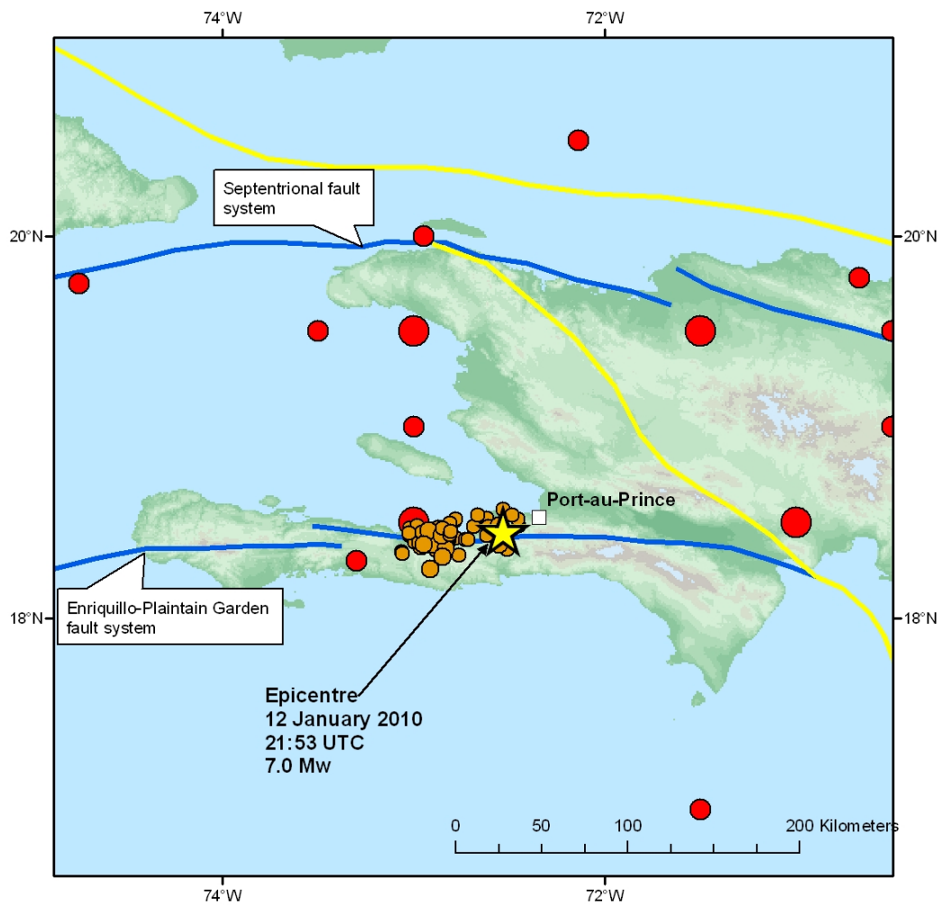
Fig. 1. The epicentre of the 12 January 2010 earthquake in Haiti (yellow star) was around 25 km west of the capital Port-au-Prince and the distribution of aftershocks (orange circles) reveals rupturing along the plate boundary over about 70 km.
