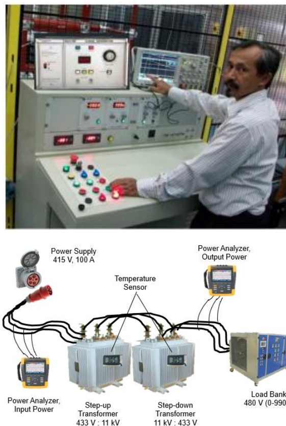
Figure 10: Circuit model for testing the performance of electric power transformers using palm oil-ester
