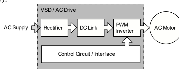
Figure 1. A typical VSD block diagram
