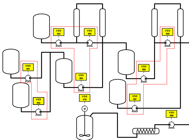
Figure 5. Typical flow diagram of the process
