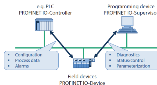
Figure 4. Communication path of Profinet IO
