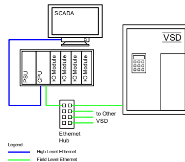
Figure 3. Typical schematic of networked control method
