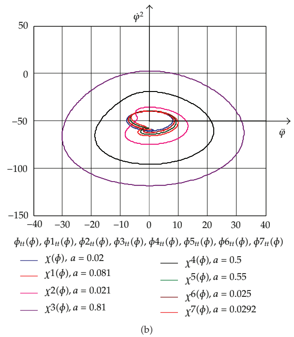
Figure 7: Transformation of the trajectory of the vector rotator \vec{\mathfrak{A}}_{022} (and \vec{\mathfrak{A}}_2 ) in the plane through pole O_2 and orthogonal to the self rotation axis, for different values of parameter a , orthogonal distance between axes of gyrorotor-disk coupled component, for rotations.
