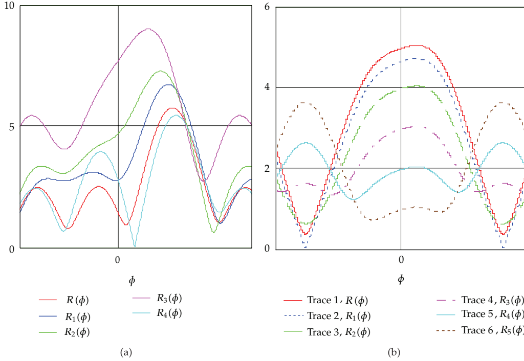
Figure 5: Intensity of vector rotators \vec{\mathfrak{R}}_{022} and \vec{\mathfrak{R}}_2 , for different disk eccentricity (a) and for different initial conditions (b).
