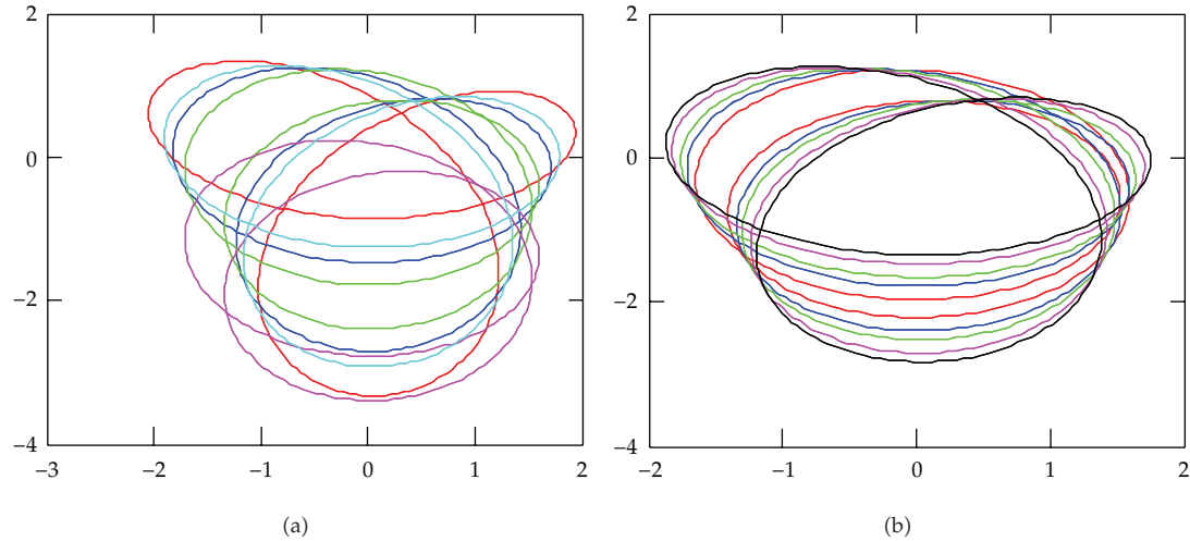
Figure 6: Transformation of the trajectory of the vector rotator \vec{\mathfrak{R}}_{022} (and \vec{\mathfrak{R}}_2 ) in the plane through pole O_2 and orthogonal to the self rotation axis for different values of parameter \psi .
