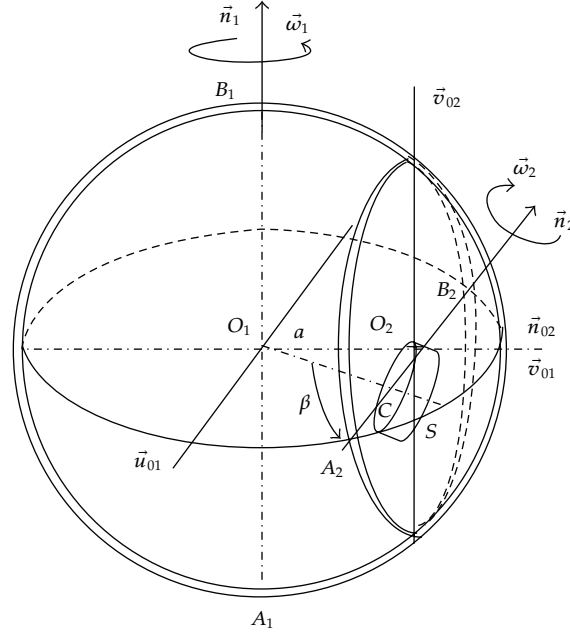
Figure 4: Model of heavy gyrorotor with two component coupled rotations around orthogonal axes without intersections.
