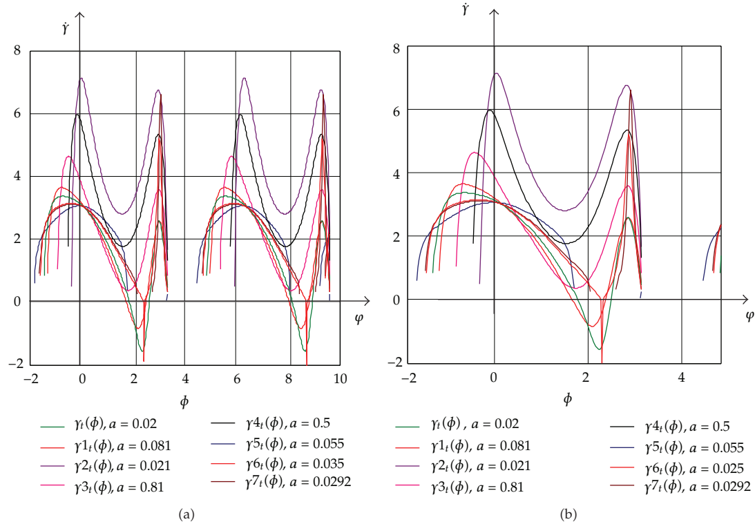
Figure 8: Relative angular velocity \dot{\gamma}_2 of the vector rotator \vec{\mathfrak{R}}_{022} (and \vec{\mathfrak{R}}_2 ) in the plane through pole O_2 and orthogonal to the self rotation axis, for different values of parameter a , orthogonal distance between axes of gyrorotor-disk coupled component rotations.
