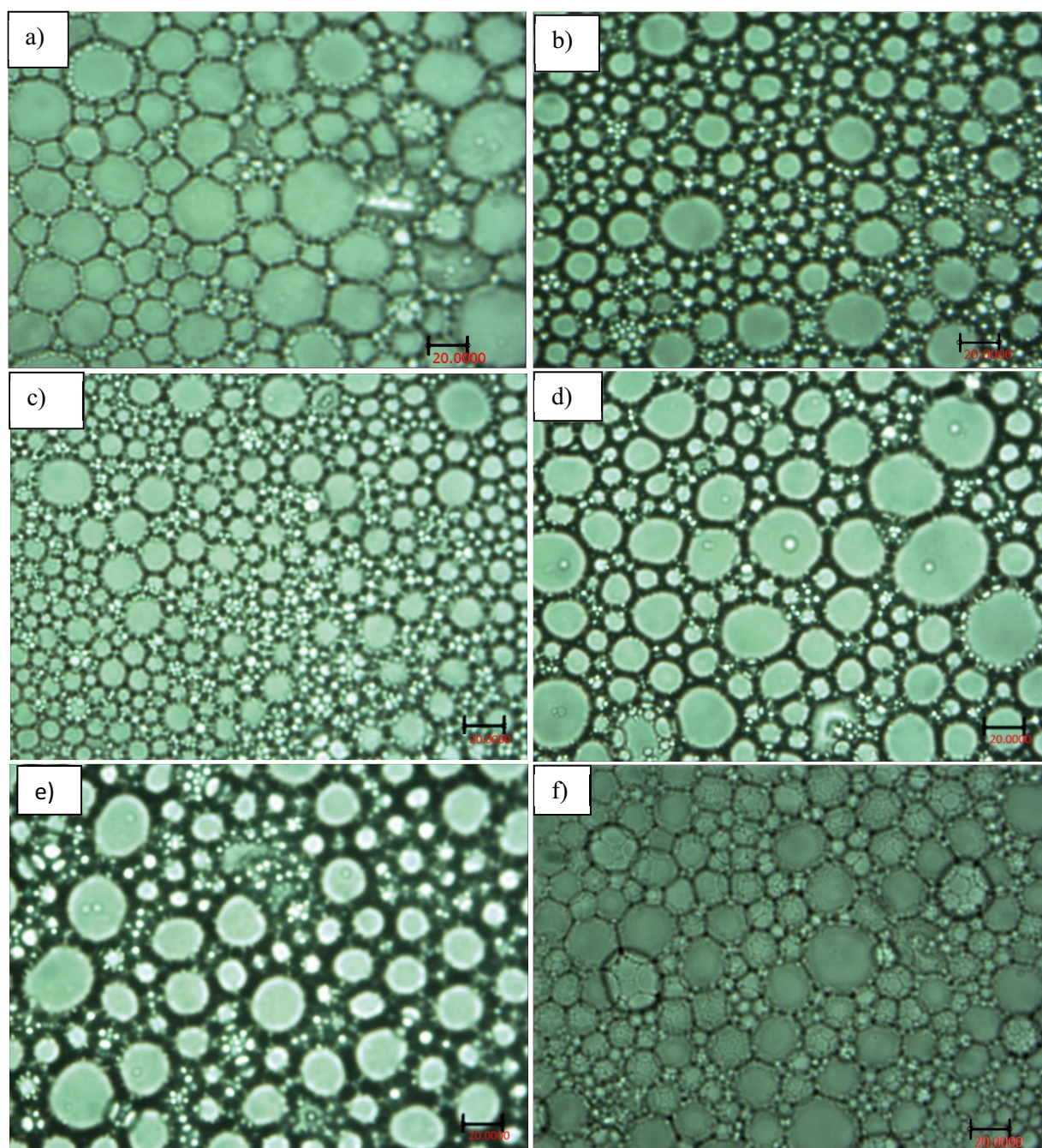
FIGURE 2. Micrographs of mayonnaise samples taken by optical microscope on the 28 th day of storage. (a) Control; (b) BHT-M; (c) \alpha -tocopherol-M; (d) 0.2% AE-MCC-AS-M; (e) 0.4% AE-MCC-AS-M; (f) 0.6% AE-MCC-AS-M
