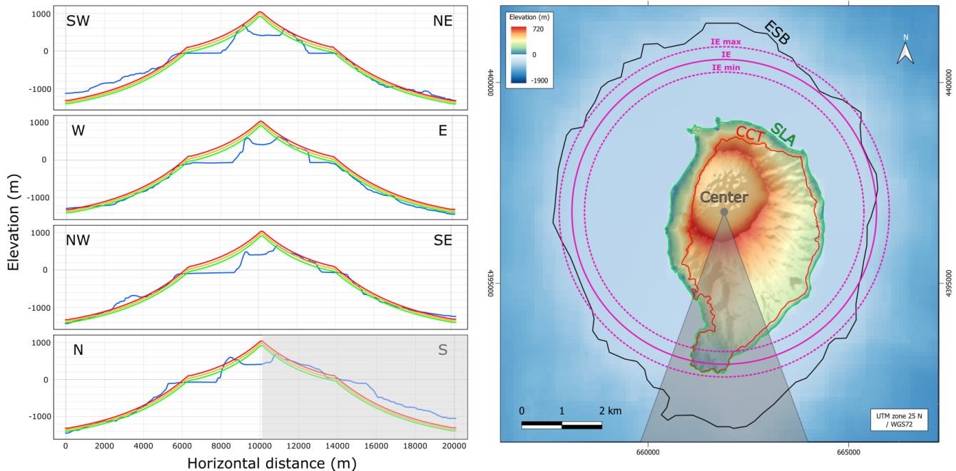
Figure 5. Left: comparison between the present-day radial topographic profiles of the Corvo volcanic edifice (blue lines) and the mean (yellow lines), minimum (green lines), and maximum (orange lines) reconstructed topographic profiles from different directions. Right: similar topographic map to the one provided in Fig. 3 (ASTER and EMODnet data) showing the initial extension of the island (solid purple line) with the uncertainty values (dashed purple lines). The gray area shows the southern sector where the volcanic progradation is located and which has been subsequently discarded for the analysis.
