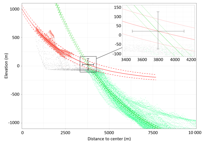
Figure 4. Elevation of the topographic data versus the distance to the center of the edifice and the initial aerial (red) and submarine (green) radial exponential profiles reconstructed with their uncertainty domain. Red dots: elevation grid points in the initial aerial domain; the red dots, found at higher elevations than all the others for the most part, belong to the northern sector. Green dots: elevation grid points in the initial submarine domain. Gray dots: data in the coastal erosion area.
