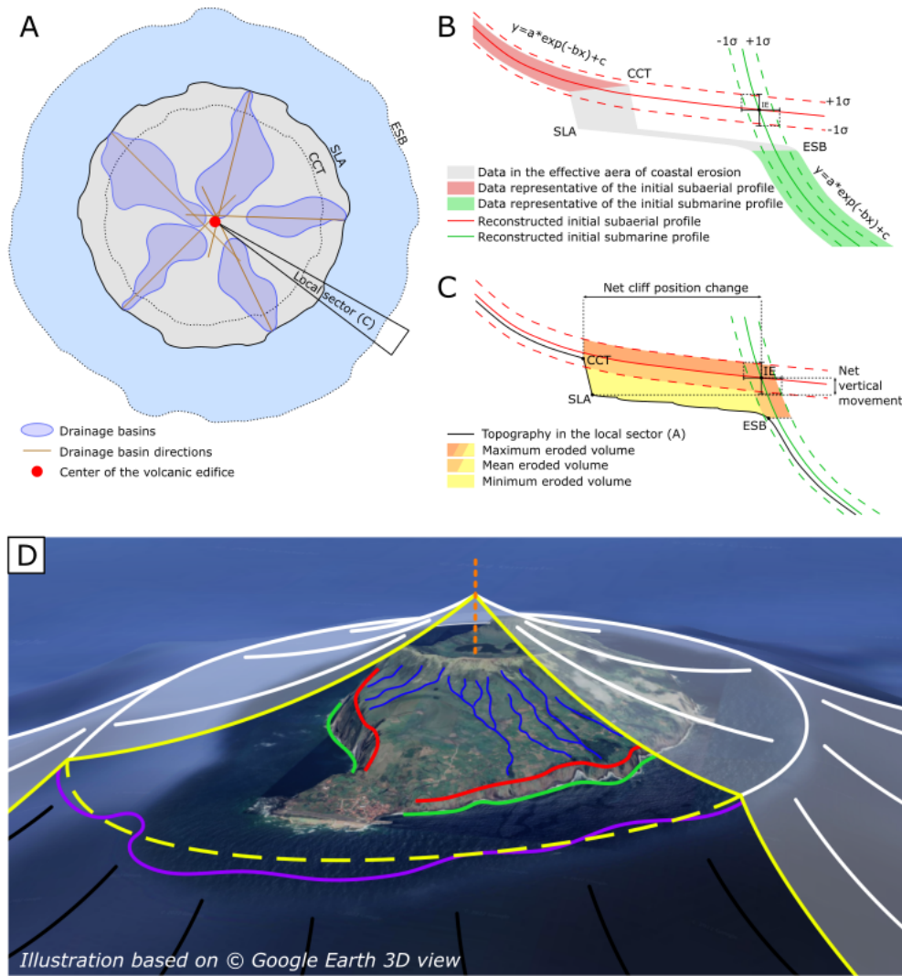
Figure 2. Topographic reconstruction method. (a) Mapping of the CCT and ESB markers and the determination of the center of the edifice. Overhead view. (b) Calculation of the radial aerial and submarine topographic profiles representative of the initial shape. (c) Quantification of the net cliff position change, eroded volume and vertical movement. (d) Illustration of the topographic reconstruction applied to Corvo Island (based on © Google Earth 3D view), as an example to better visualize the eroded volume below the reconstructed shape (yellow) and between the CCT (red) and the ESB (purple).
