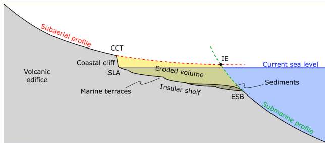
Figure 1. Schematic representation of a radial topographic profile of a volcanic island. The initial aerial and submarine profiles are demarcated with dashed lines. CCT: coastal cliff top. SLA: shoreline angle. ESB: erosional shelf break. IE: initial extension. Note the presence of marine terraces, corresponding to different low eustatic levels, and sediments on the insular shelf.
