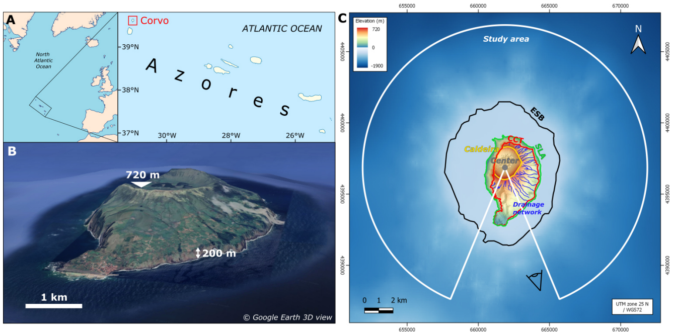
Figure 3. (a) Location of Corvo Island. (b) Corvo Island seen from the southeast (© Google Earth 3D view). C: topographic shaded relief map of the volcanic edifice of Corvo (ASTER and EMODnet data). White line: study area. Black line: ESB. Green line: coastline, SLA. Red line: CCT. Yellow line: edges of the central volcano caldera. Blue lines: drainage network on the slopes of the central volcano. Gray dot: center of the volcanic edifice.
