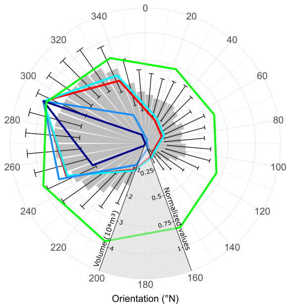
Figure 6. Total eroded volume (gray columns) with respect to direction. The wave data from Rusu and Guedes Soares (2012) are shown in color and in values normalized by their maximum (see Tables 2 and 3 for the detailed actual values). Red: spatial distribution for the waves. Light blue: spatial distribution for the waves with H_s < 5 m. Blue: spatial distribution for the waves with 5 \text{ m} < H_s < 10 m. Dark blue: spatial distribution for the waves with H_s > 10 m. Green: mean H_s of the waves.
