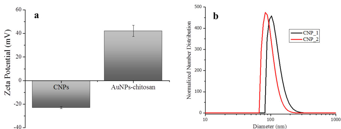
Figure 4. (a) Zeta potential for gold–chitosan (AuNPs–chitosan) and carbon nanoparticles (CNPs); (b) dynamic light scattering of the synthesized CNPs.
