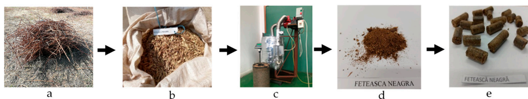
Figure 1. Simplified scheme of the pellets production process from vineyard wastes: (a) vineyard wastes; (b) course grinding; (c) drying; (d) fine grinding; and (e) pelletization.
