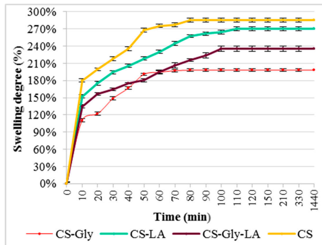
Figure 6. Swelling degree (%) in distilled water.
