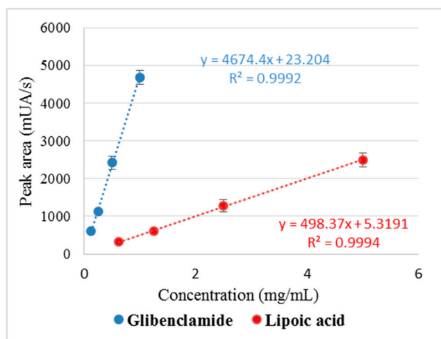
Figure 3. Standard curve and correlation coefficient ( R^2 ) values for glibenclamide and lipoic acid.
