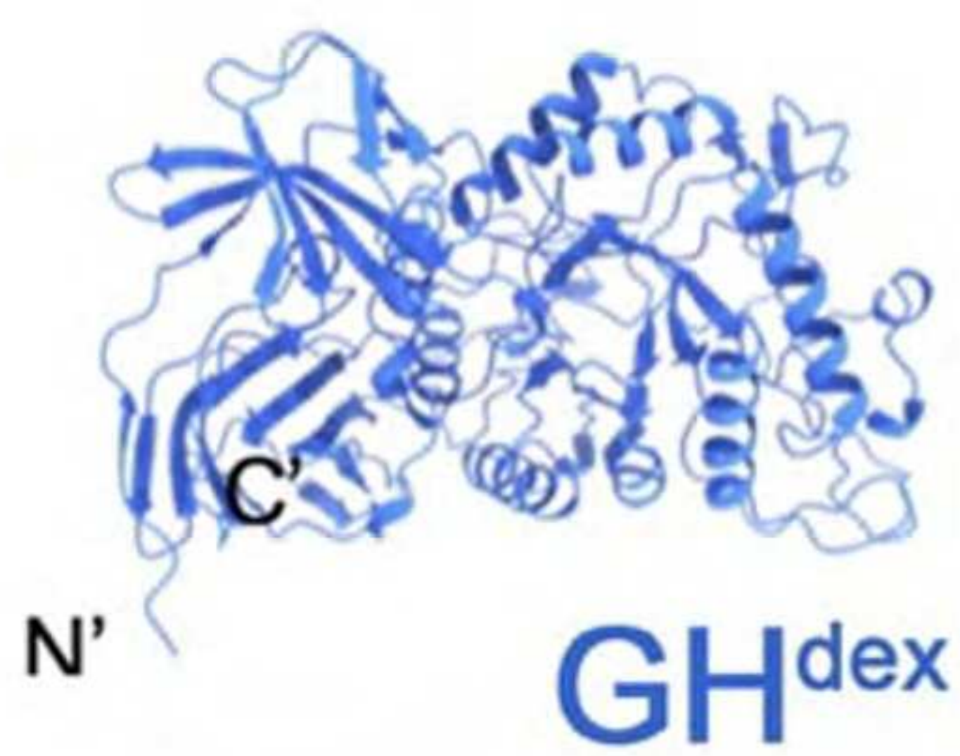
AlphaFold prediction
