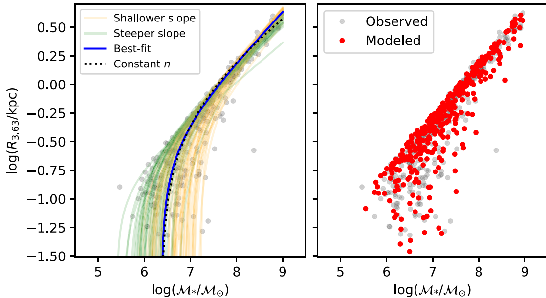
Figure 4. Tests demonstrating the nature of the theoretical IRSMR. The left panel shows our fiducial IRSMR, for galaxies with masses below \mathcal{M}_* < 10^9 \mathcal{M}_\odot . We show our best-fitting curve predicted from our log-linear fits to the \mathcal{M}_*-n and \mathcal{M}_*-\Sigma_{*,0} relations (Table 1) in blue. The orange and green lines show predicted curves in this space made by adjusting our best-fitting slopes and intercepts by the error on the fit parameters in Table 1, demonstrating the sensitivity of the curve’s shape to the parameters. The green lines have steeper slopes in the \mathcal{M}_*-\Sigma_{*,0} relation, while the orange lines have shallower slopes in this relation. For comparison, we show the curve predicted assuming a constant value of n as a dotted black line, which is almost indistinguishable from our best-fitting relation. We plot the observed IRSMR for FDS dwarfs as black points underneath. The right panel shows the observed IRSMR for FDS dwarfs in black, while the red points show a theoretical IRSMR made by adding artificial scatter about the best-fitting \mathcal{M}_*-n and \mathcal{M}_*-\Sigma_{*,0} relations before deriving the isomass radii from them. The scatter here is preferentially downward, just as it is in the observed relation.
