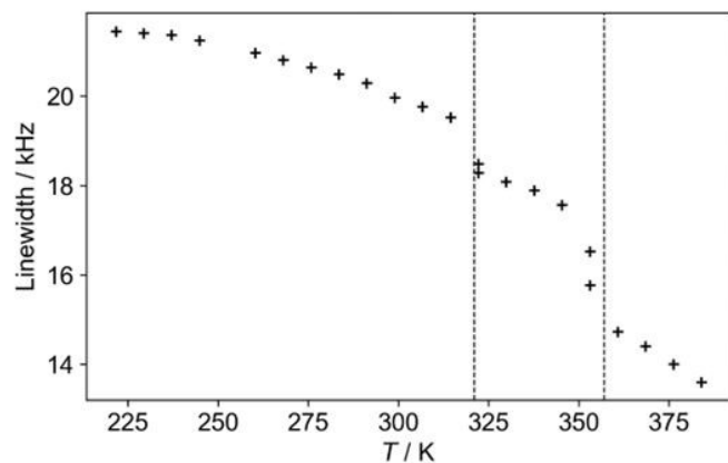
Fig. 5: Static ^1\text{H} NMR linewidth of [\text{NH}_3\text{NH}_2]\text{Mg}(\text{HCO}_3)_2 as a function of temperature.
