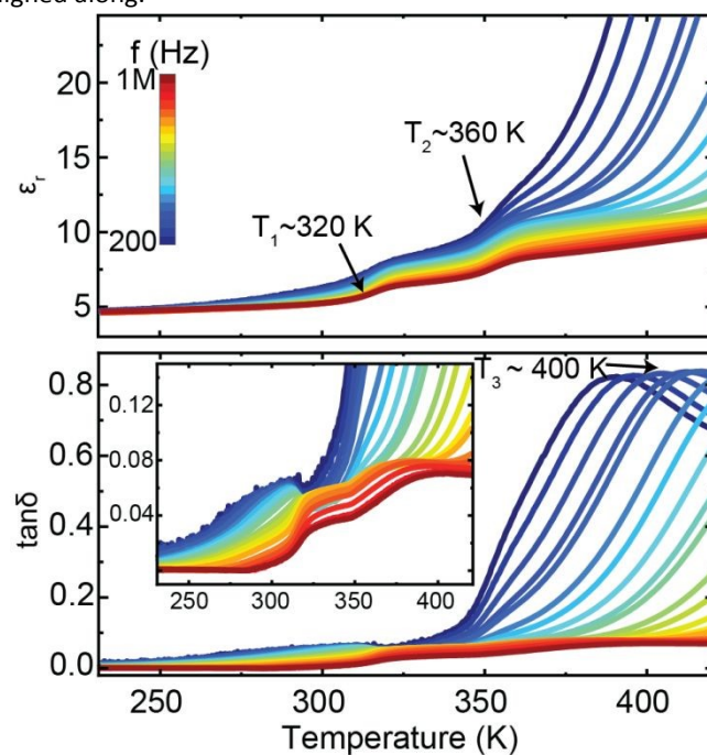
Fig. 8: Temperature-dependent dielectric constant ( \epsilon' ) and losses ( \tan\delta ) of [\text{NH}_3\text{NH}_2]\text{Mg}(\text{HCO}_2)_3 . The inset is the enlargement of the dielectric losses.
