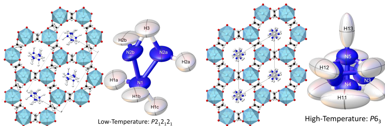
Fig. 1: The crystal structure of [\text{NH}_3\text{NH}_2]\text{Mg}(\text{HCO}_2)_3 , modelled from the single crystal neutron diffraction in both the orthorhombic low-temperature phase at 250 K and the hexagonal high-temperature phase at 400 K, with the cation disorder shown for clarity to the right of each structure. At high temperature N3 atoms lie in a plane perpendicular to the c-axis generated by the six-fold screw axis along which N4, N5 and H13 sit. The atom labelled N3 in the figure is at the equivalent general positions (\bar{x} + y, \bar{x}, z) .
