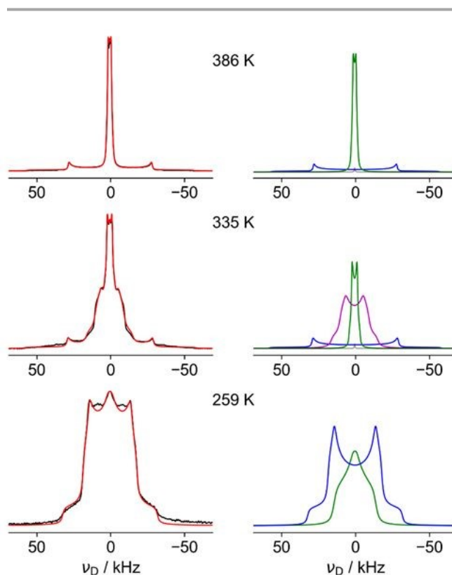
Fig. 4: Fitting of representative ^2\text{H} NMR spectra of [\text{ND}_3\text{ND}_2]\text{Mg}(\text{HCO}_2)_3 from low, intermediate and high temperature regions. (Left) experimental spectra (black) and overall fittings (red). (Right) Individual fitting components: (blue) high C_Q , (green) low C_Q . Additional components were required in some fittings: (purple) intermediate C_Q and (grey) small zero-frequency artefact.
