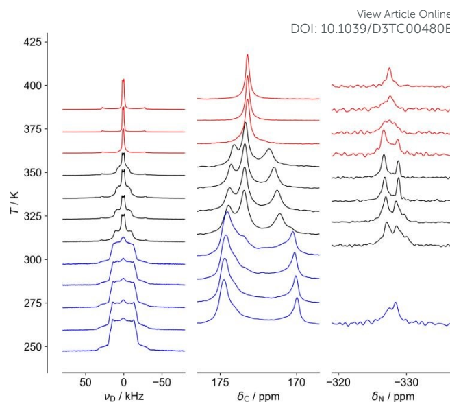
Fig. 3: NMR spectra as a function of temperature (baseline of each spectrum indicates sample temperature). Left: ^2\text{H} spectra of [\text{ND}_3\text{ND}_2]\text{Mg}(\text{HCO}_2)_3 . Centre: ^{13}\text{C} spectra of [\text{ND}_3\text{ND}_2]\text{Mg}(\text{HCO}_2)_3 . Right: ^{15}\text{N} spectra of [\text{NH}_3\text{NH}_2]\text{Mg}(\text{HCO}_2)_3 . The three distinct temperature regimes observed are highlighted using colour: (red) high temperature phase, (blue) low temperature phase, (black) intermediate regime.
