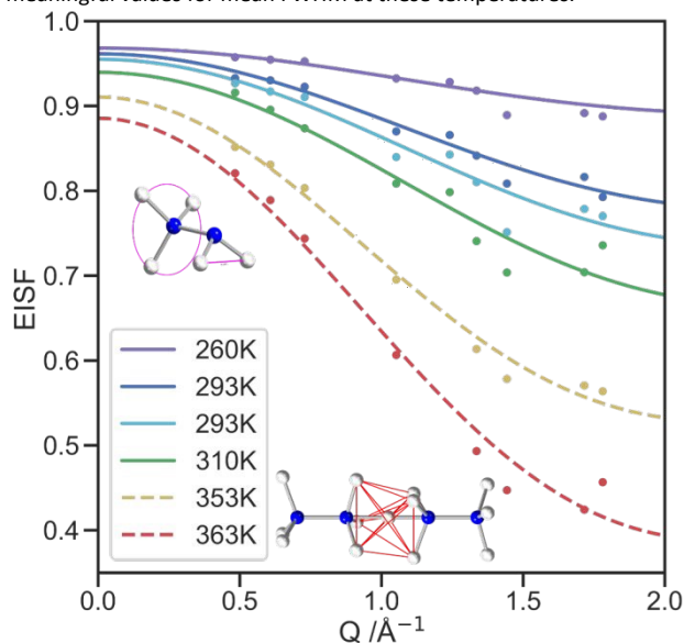
Fig. 7: EISF data collected in the PG(002) configuration and associated models for low temperature in solid lines and high temperature in dashed lines. Visual representations of the low temperature (magenta) and high temperature (red) site exchanges are overlaid.
