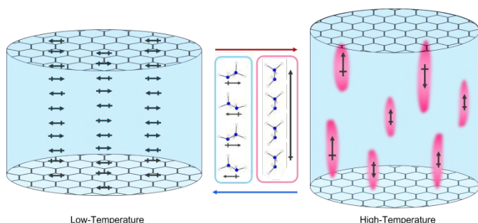
Fig. 9: Visualisation of (left) antiparallel dipoles in the anti-ferroelectric low-temperature phase (blue). Right) the high temperature phase with dynamic polar nanoregions (pink), with dipoles aligned along the polar axis, amongst the bulk non-polar dipoles (blue). The distortion of the framework is also alluded to in the lengthening of the channel direction and contraction of the pore diameter.
