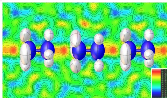
Fig. 2: Fourier difference map showing the experimentally observed nodes of negative scattering (red) between the modelled \text{NH}_2\text{NH}_3^+ cation chains. The proton site between cations is omitted to display the residual negative scattering. The rest of the difference map shows the experimental background that exhibits a combination of low-intensity residual positive (blue-green) and negative (orange-yellow) scattering.
