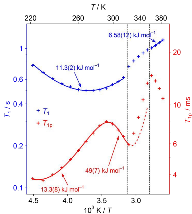
Fig. 6: ^1\text{H} T_1 (blue) and T_{1p} (red) relaxation time constants as a function of temperature. Error bars are not shown as they are of a similar magnitude to the size of symbols used. Curves show fits to relaxation models (see Supplementary Information for details of the fittings). The straight line fit in the HT phase is a guide for the eye and this E_a value should be interpreted cautiously. The data is not fitted in the transition region since the material is changing; the dashed line extrapolates the behaviour from the low temperature region fit.
