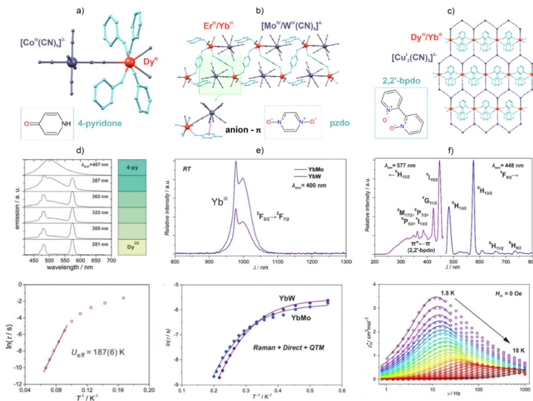
Fig. 8 (a) Structural view of the \{[Dy^{III}(4\text{-pyridone})_4(H_2O)_2][Co^{III}(CN)_6]\cdot nH_2O dinuclear molecule (where an analogous structure is observed for the Rh III -based derivative), 223 and (d) its excitation-wavelength-dependent emission spectra with the depicted emission colours (top), shown together with the temperature-variable magnetic relaxation times for the zero-dc-field (bottom). (b) Structural view of the (PPN)[Ln III (pzdo) 2 (MeOH) 0.3 (H 2 O) 3.7 ][M IV (CN) 8 ] \cdot 7.7H 2 O \cdot 2MeOH coordination chains (Ln = Er, Yb; M = Mo, W; pzdo = pyrazine N,N' -dioxide; PPN = bis(triphenylphosphine)iminium), 224 and (e) the emission spectra for the related {YbMo} and {YbW} chains (top) shown together with the temperature-variable magnetic relaxation times for these compounds (bottom). (c) Structural view of the [Ln III (2,2'-bpdo) 2 (H 2 O)] [Cu 2 (CN) 5 ] \cdot 5H 2 O coordination networks (Ln = Dy, Yb; 2,2'-bpdo = 2,2'-bipyridine N,N' -dioxide; view of the layered part of the network), 225 and (f) the excitation and emission spectrum of the {DyCu} framework at 77 K (top), and its representative ac magnetic characteristics (bottom). Part (d) was reproduced from ref. 223 with permission from the Royal Society of Chemistry. Part (e) was reproduced from ref. 224 with permission from the Royal Society of Chemistry. Part (f) was adapted with permission from ref. 225. Copyright 2019 John Wiley & Sons.
