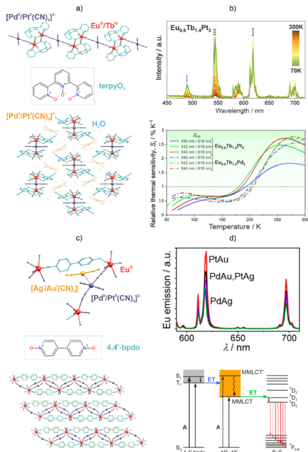
Fig. 6 (a) Structural view of the \{[Ln^{III}(H_2O)_4(terpyO_3)_2[M^{II}(CN)_4]_2]_n \cdot 8H_2O (Ln = Eu, Tb; M = Pt, Pd; terpyO 3 = 2,2':6',2''-terpyridine N,N',N'' -trioxide) coordination chains, 218 (b) temperature-variable emission spectra for the \{Eu_{0.6}Tb_{1.4}Pt_3\} analogue under 323 nm excitation (top), shown together with the temperature dependence of the relative thermal sensitivity for two representative compounds under the indicated excitation conditions (bottom). (c) Structural view of the \{[Eu^{III}(4,4'-bpdo)(H_2O)_2][M^{II}(CN)_4]\} \cdot [M'(CN)_2] \cdot H_2O (M II = Pt II , Pd II ; M' = Au I , Ag I ; 4,4'-bpdo = 4,4'-bipyridine N,N' -dioxide) layered coordination networks, 219 (d) their emission spectra for various d 8 –d 10 metal combinations (top), and the schematic energy level diagram depicting the nature of the electronic transitions and energy-transfer processes (bottom). Part (b) was reproduced from ref. 218 with permission from the Royal Society of Chemistry. Part (d) was adapted with permission from ref. 219. Copyright 2020 American Chemical Society.
