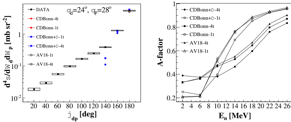
Figure 3: (Color online) Left panel: Differential, but integrated over S , cross section presented as a function of the relative azimuthal angle \varphi_{dp} , for a given \theta_d, \theta_p combination as indicated in the panel. The data points are compared with the results of calculations based on pure CD Bonn, Argonne V18 and CD Bonn+ \Delta potentials for 1-term (1t) and 4-term (4t), as described in the legend. The boxes around the experimental points represent the total systematic errors. Right panel: Quality of the description of the cross-section data with various theoretical predictions (defined in the legend), expressed as a dependence of the A-factor on the neutron energy E_n . The bin size was chosen to be \pm 2 MeV. Lines connecting points are used to guide the eye. For details see also Refs. [37, 38].
