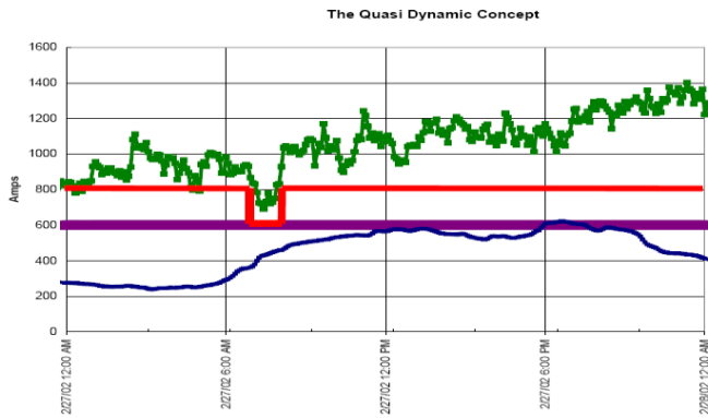
Figure 1. The operating regions generated by the quasi-dynamic scenario adopted from [1]
