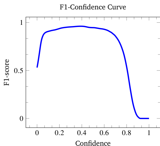
Fig. 6 F1-Confidence Curve of pre-trained YOLOv5l with an input size of 1280px × 1280px on the validation set. Each point on the line indicates the F1-score at the given confidence filter constant. The peak of the F1-score is 0.97, reached at the confidence of 0.475.
