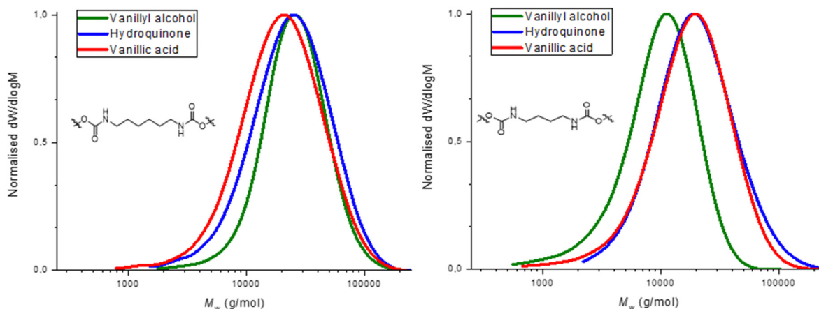
Fig. 2 GPC traces of the different PHUs obtained from functionalized vanillin bis-carbonates.
