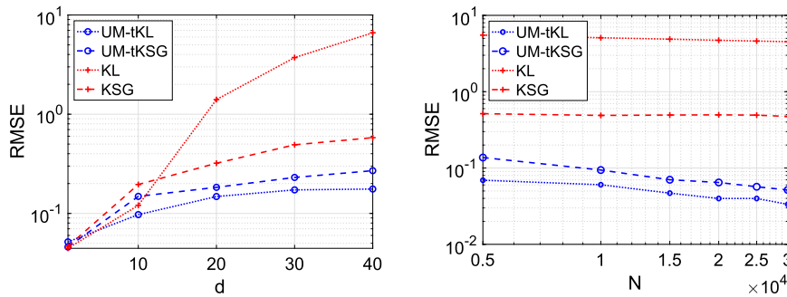
Fig. 3. Left: RMSE plotted against the dimensionality d . Right: RMSE (on a logarithmic scale) plotted against the sample size N .
