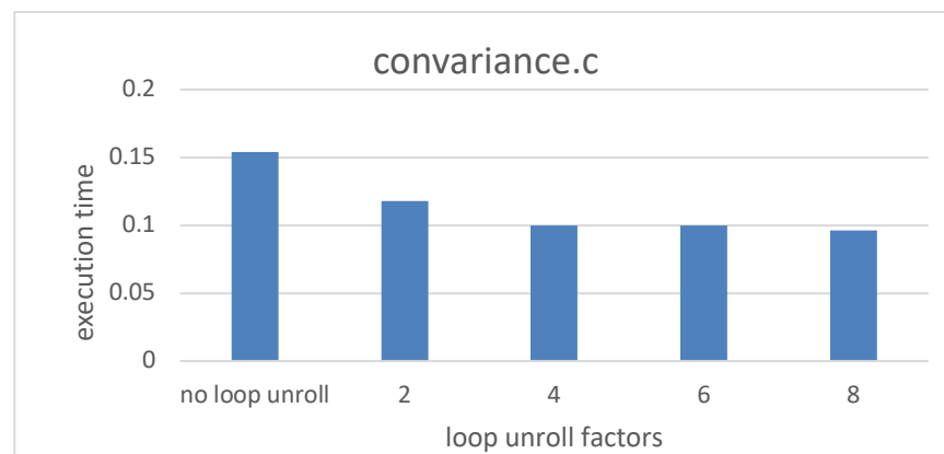
Fig. 5: illustrates the predicted factor for convariance.c program
