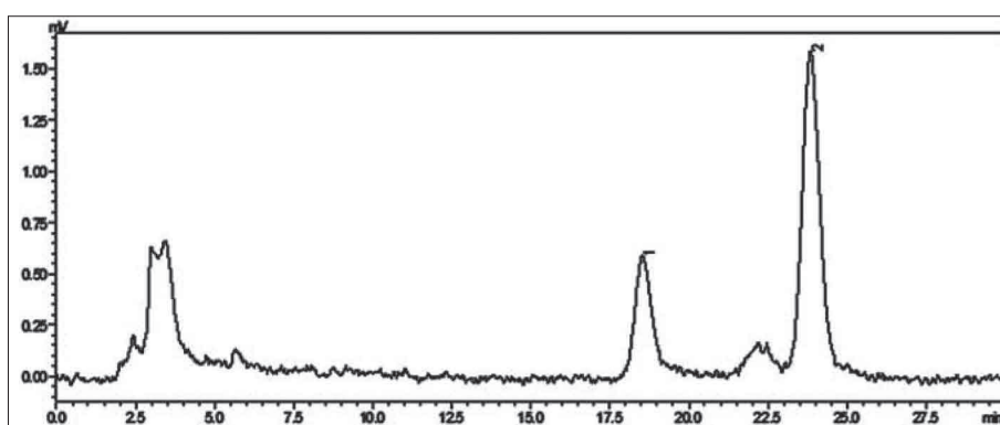
Fig 2. HPLC-FLD chromatogram of the aflatoxin positive sample, 1- AFB 2 , 2- AFB 1
