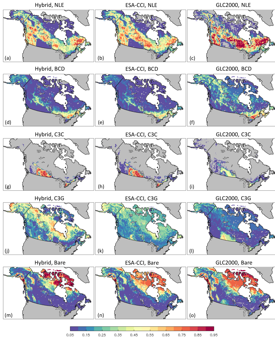
Figure 3. The spatial distribution of CLASSIC PFTs based on the hybrid (left), ESA-CCI (middle), and GLC2000 (right) land cover datasets respectively. The maps for C_4C and C_4G are not shown for their fractions are small (0.5 % for C_4 crops and 0.1 % for C_4 grasses) in Canada. The last panel shows fractions for bare ground from the three datasets.
