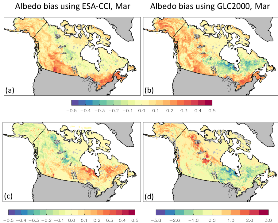
Figure 5. Surface albedo bias (relative to MODIS) in CLASSIC simulations using PFT distributions based on (a) ESA-CCI and (b) GLC2000 land cover products. Panels (c) and (d) show the difference in simulated surface albedo (c) and leaf area index (d) between the two simulations.
