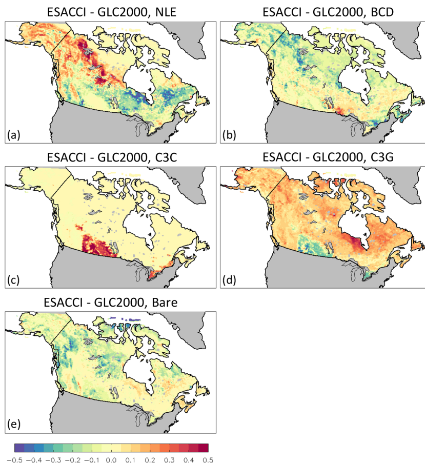
Figure 4. The difference in PFTs based on ESA-CCI and GLC2000 datasets for selected PFTs (a) NLE, (b) BCD, (c) C 3 C, (d) C 3 G, and (e) bare.
