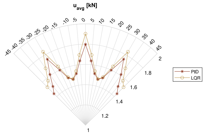
Fig. 14. Polar plot showing the average thrust expended by the controllers.
