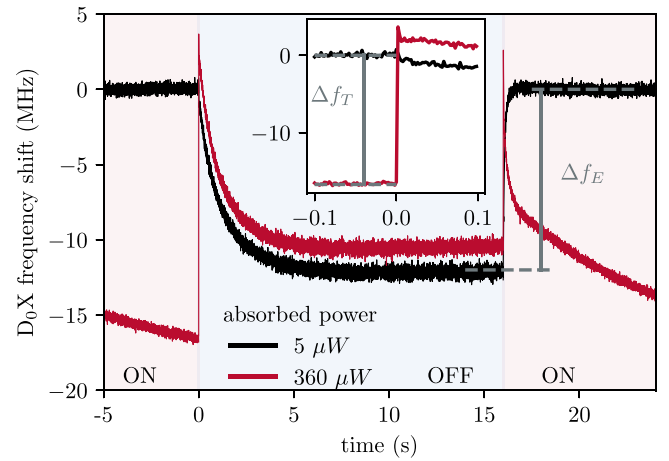
FIG. 3. Temporal shift of the \text{D}^0\text{X} resonance frequency for 5 \mu\text{W} (black line) and 360 \mu\text{W} (red line) ABE power, respectively. The ABE is periodically switched on and off periodically for 16 s whereat the moment of switching off defines t = 0 . The complete dynamics results from changes of temperature, changes of the charge states of donors and acceptors, and long-living surface electric fields at which \Delta f_T is the frequency change due to the temperature change and \Delta f_E is the frequency change due to the change of the electric field induced by neutralizing the ionized donors and acceptors.
