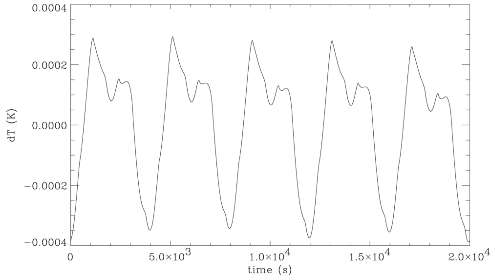
Figure 6. Time ordered data representing the 30 GHz radiometric output caused by a fluctuation in the 4 K reference signal induced by LR1 temperature variations (coupled scheme, see Figure 2).
