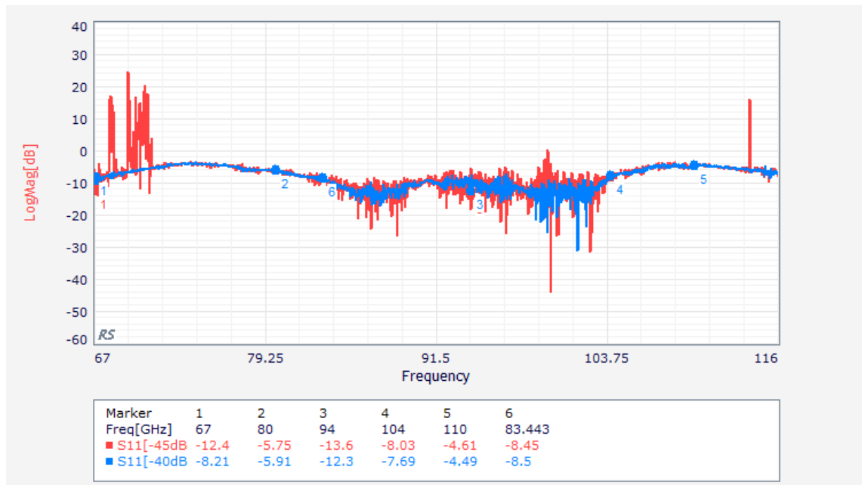
Figure 27 RL: S220 has nominal bias ; VNA input level is decreased from -45 dBm to -40 dBm.
