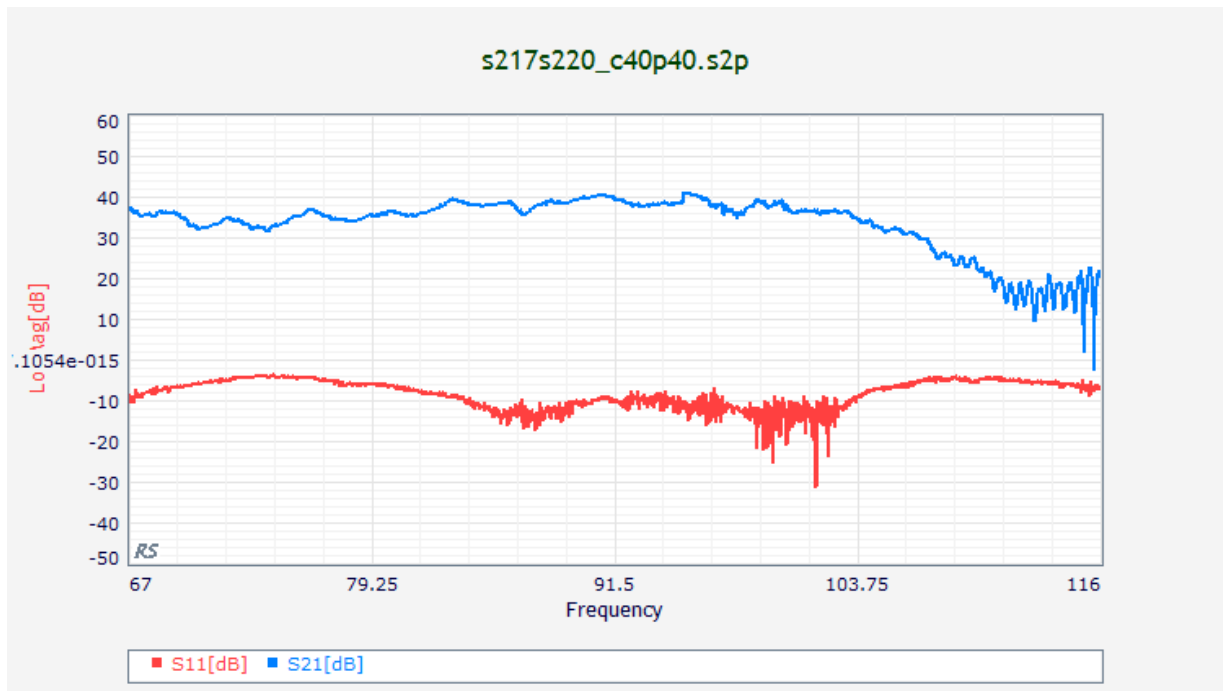
Figure 22 cascaded S217 and S220 LNAs: nominal bias setup with Input level increased from -45 dBm to -40 dBm.
