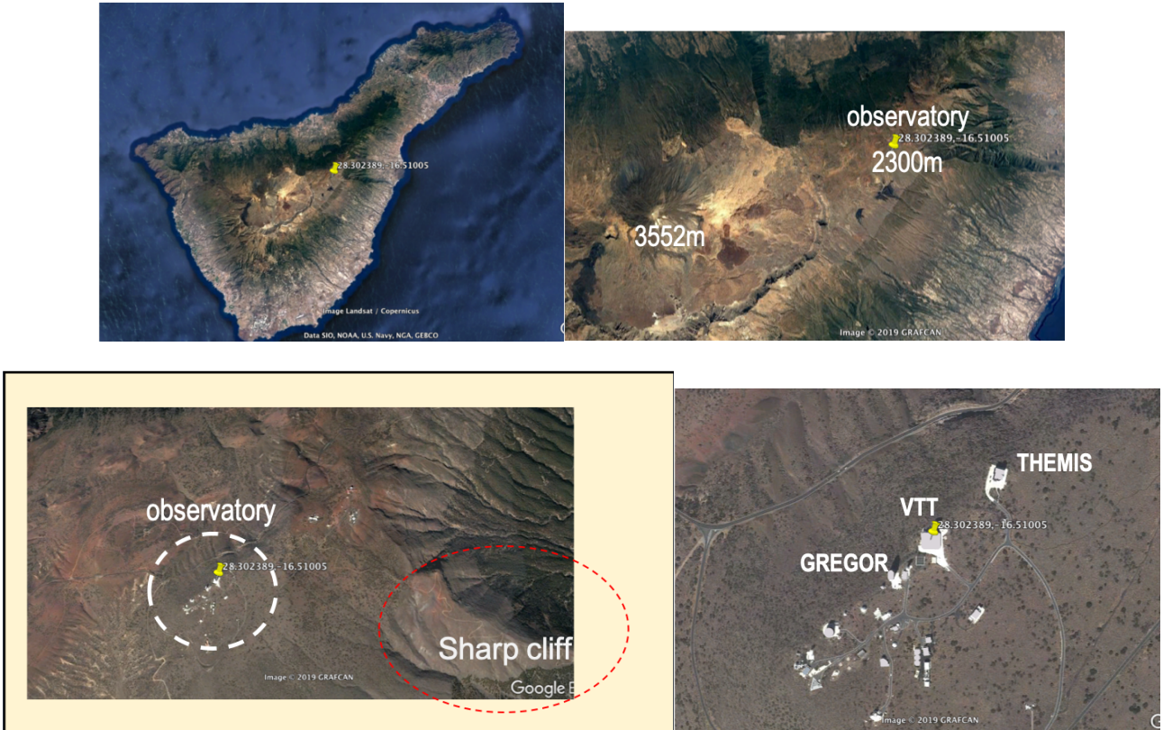
Fig. 10: Top-left: satellite view of the Tenerife Isle. Top-right: zoom of the region around the Teide Observatory in which it is visible a mountain on the West-side that is ~ 1 km higher than the TO summit. Bottom-left: a sharp cliff at the East with respect to the Teide Observatory. Bottom-right: position of the Vacuum Tower Telescope (VTT).
