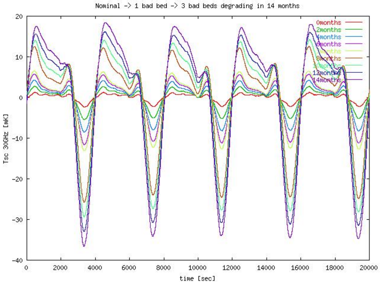
Figure 10 Simulated degradation of T_{sc,30GHz} for the case of a system degrading from the nominal case to 1 bad bed in the first 7 months (curves from red to yellow) and from 1 bad bed to 3 bad beds in the remaining 7 months (from yellow to black).
