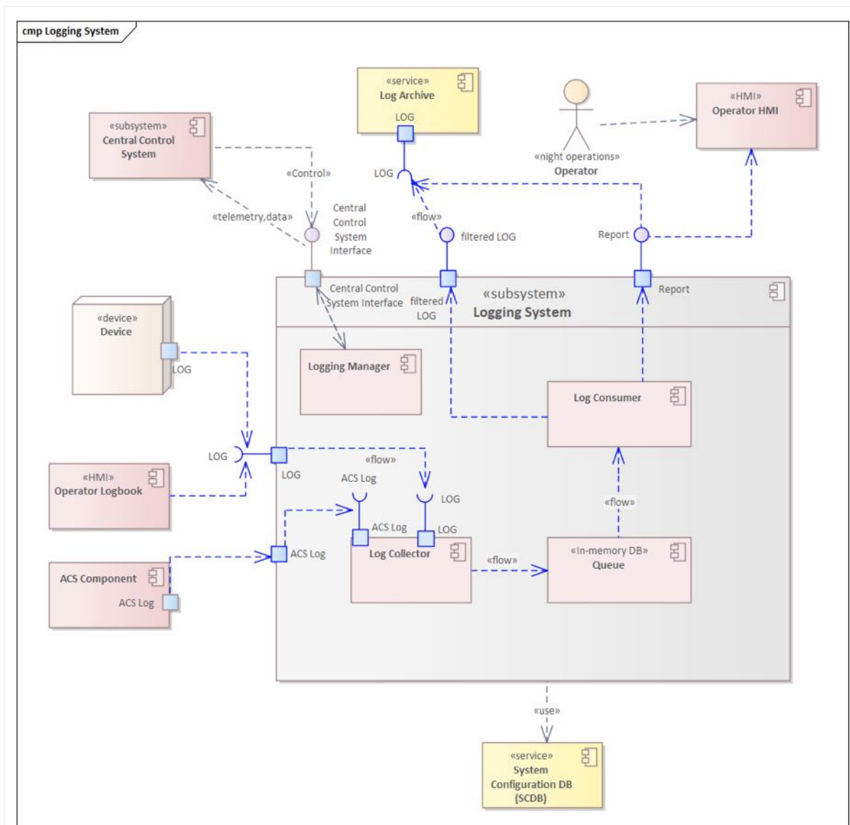
Figure 41: The Logging System. The Logging Manager coordinates the workflow.
