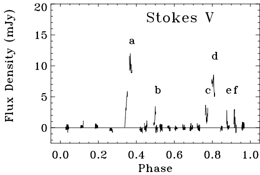
Fig. 5. Stokes parameter V versus rotational phase in the 3 days of observation. No polarization is seen outside the peaks denoted with the letters from a to f . The higher fluxes ( a and d ) are visible when the magnetic axis is perpendicular to the line of sight.
