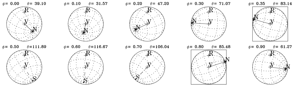
Fig. 8. Changes of the geometry of CU Vir as a function of the rotational phase. The point V at the center of the star is the intersection of the stellar surface with the line of view; the point R close to the top is the rotational pole; the points denoted with N and S represent the North and South magnetic poles; the arc V-N subtends the angle \theta_M . \phi and \theta_M are indicated in each panel. The main peaks are visible when the star is oriented as in the two framed panels at \phi \approx 0.35 (peak a) and at \phi \approx 0.80 (peak d).
