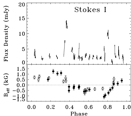
Fig. 4. Upper panel: 1.4 GHz emission from CU Vir; Lower panel: Longitudinal magnetic field measurements from Borra & Landstreet (1980) and from Pyper et al. (1998) (open and filled circles respectively) as a function of the rotational phase. 1.4 GHz radiation maxima correspond approximately with the null magnetic field.
