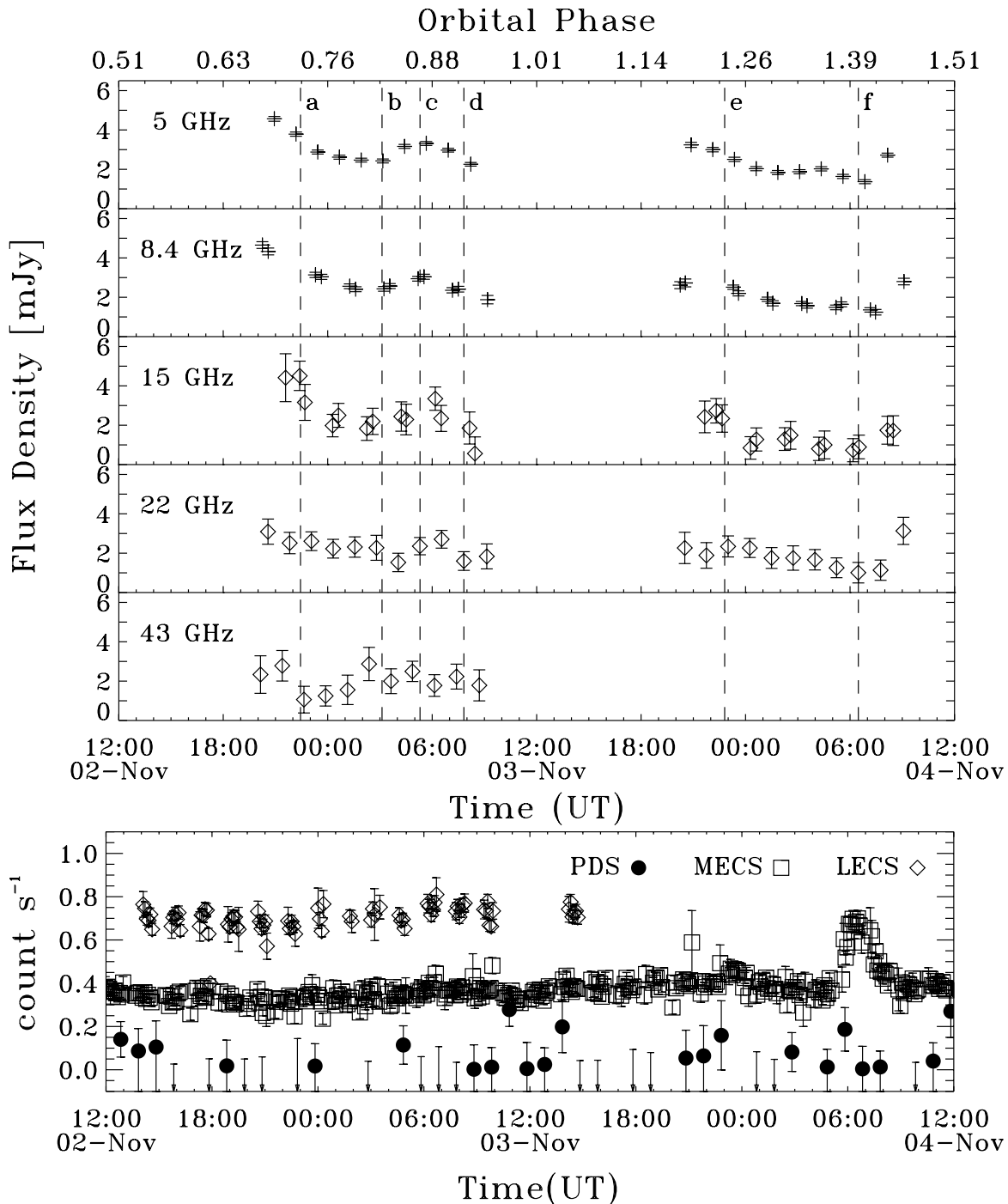
Fig. 1. Top panel: VLA flux curves of AR Lac binned over 20 min. Dot-dashed vertical lines indicate the times of the spectra labelled by the letters on the top and shown in Fig. 2. Lower panel: the contemporaneous SAX light curves (from Rodonò et al. 1999).
