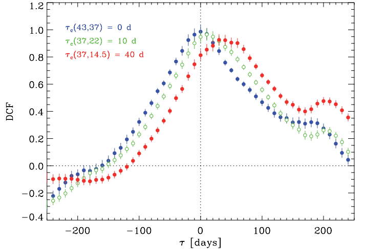
Fig. 2. Discrete correlation functions (DCFs) between radio light curves: 43 versus 37 GHz (blue filled circles), 37 versus 22 GHz (green empty circles), and 37 versus 14.5 GHz (red filled circles).
