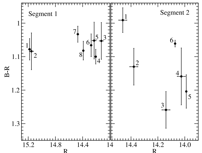
FIG. 5.— Color-magnitude diagrams for the two time segments marked in Fig. 2, with time ordering indicated by the numbers in the two panels.
