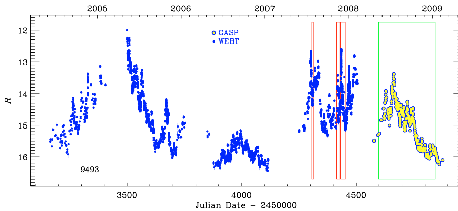
Fig. 1. R -band light curve of 3C 454.3 in the last five observing seasons, composed with data from the WEBT campaigns (blue dots) and from the GASP monitoring (yellow-filled circles); the boxes indicate various periods of \gamma -ray detection, as described in the text.
