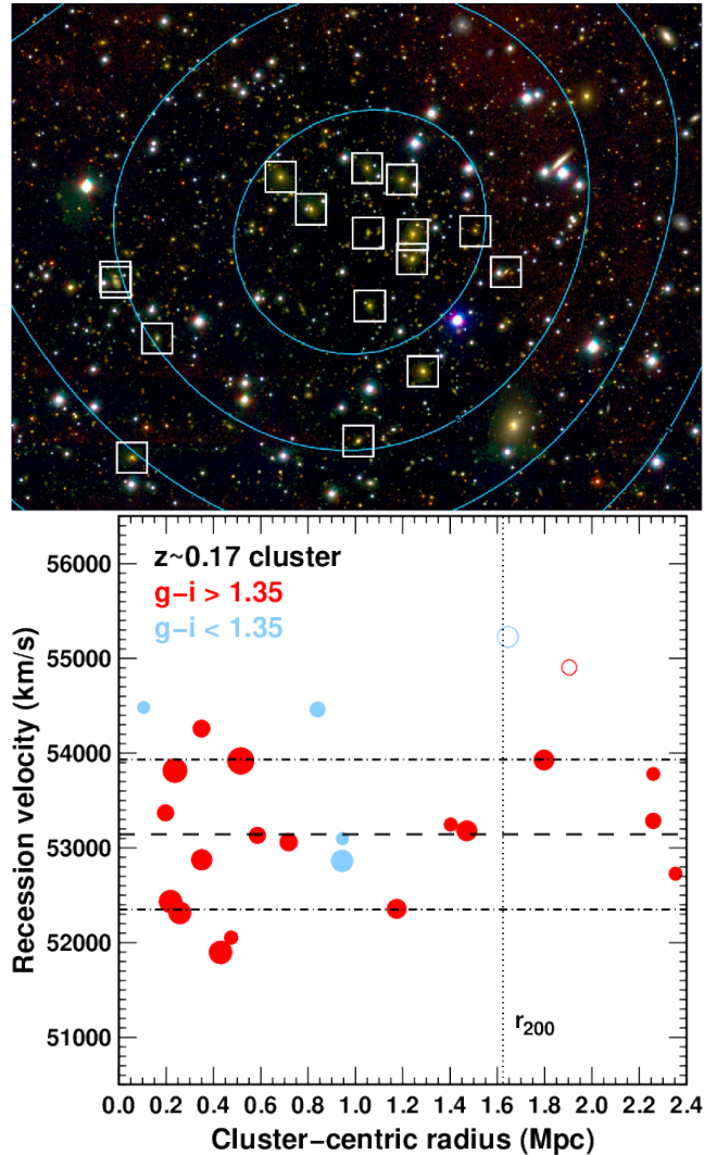
Figure 9. Upper panel: gri colour composite image centred on the WL detection (blue contours) of a background cluster at redshift z \sim 0.17 . The blue contours indicate the WL peak. Lower panel: Distribution of cluster members of the background cluster (solid dots, sizes scale with i -band luminosity) and non-members (open circles) in the caustic diagram; line-of-sight velocity, cz , versus projected distance from the centre of the WL peak. The dashed and dot-dashed lines indicate the central velocity and 1\sigma velocity dispersion of member galaxies within r_{200} (vertical dotted line).
