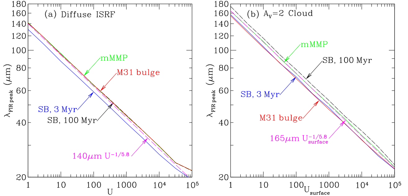
Figure 13. Wavelength \lambda_{\text{FIR peak}} where \lambda_j peaks in the far-infrared, as a function of starlight heating parameter U , for our standard model and various radiation fields. (a) Unattenuated radiation fields. (b) Emission summed over a cloud with A_V = 2 . In each panel, the magenta dashed line is a power-law fit.
