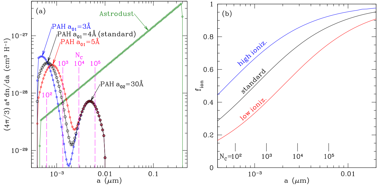
Figure 9. (a) Size distributions for astroduct and PAHs, for three different values of parameter a_{01} (see the text). Sizes corresponding to N_C = 10^2, 10^3, 10^4, and 10^5 are indicated. The dots show the discrete sizes used in our modeling. (b) Three examples of PAH ionization fractions (see the text).
